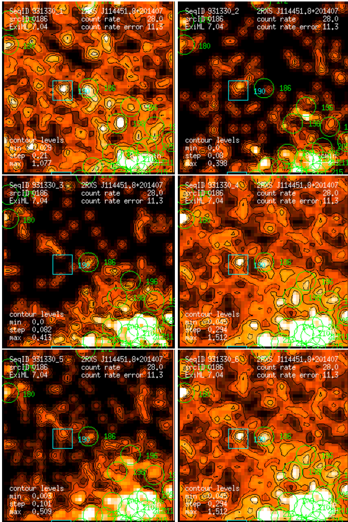
Figure 186: RASS 931330: detection 0186: band rate images, Gaussian filter: (1) PSPC channels 11 – 41, (2) 52 – 90, (3) 91 – 201, (4) 11 – 235, (5) 52 – 201, (6) 11 – 201. Broad band rates in counts/ks. Band rate contour levels in counts/ks/arcmin 2 .
