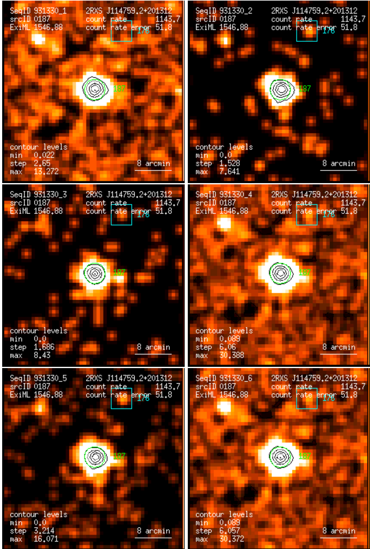
Figure 187: RASS 931330: detection 0187: band rate images, Gaussian filter: (1) PSPC channels 11 – 41, (2) 52 – 90, (3) 91 – 201, (4) 11 – 235, (5) 52 – 201, (6) 11 – 201. Broad band rates in counts/ks. Band rate contour levels in counts/ks/arcmin 2 .
