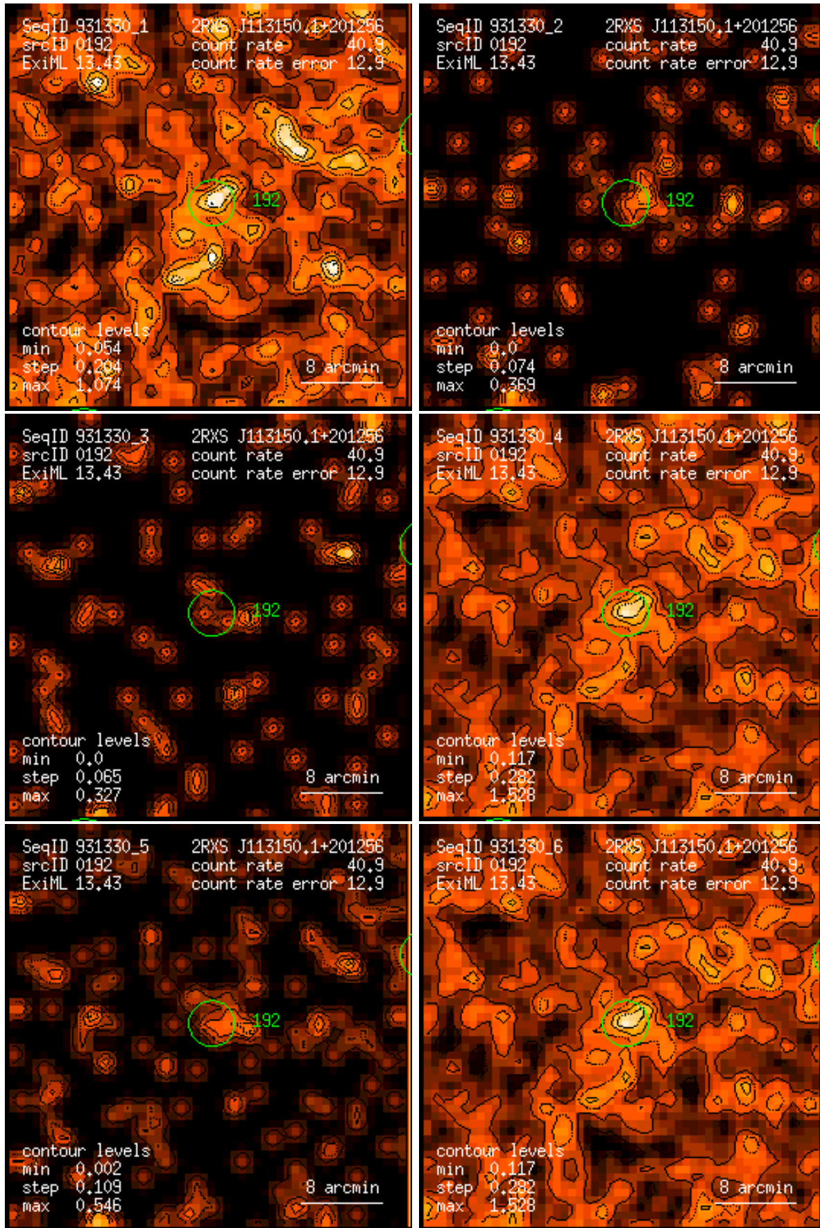
Figure 192: RASS 931330: detection 0192: band rate images, Gaussian filter: (1) PSPC channels 11 – 41, (2) 52 – 90, (3) 91 – 201, (4) 11 – 235, (5) 52 – 201, (6) 11 – 201. Broad band rates in counts/ks. Band rate contour levels in counts/ks/arcmin 2 .
