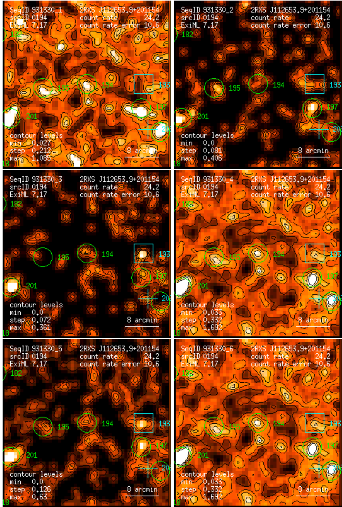
Figure 194: RASS 931330: detection 0194: band rate images, Gaussian filter: (1) PSPC channels 11 – 41, (2) 52 – 90, (3) 91 – 201, (4) 11 – 235, (5) 52 – 201, (6) 11 – 201. Broad band rates in counts/ks. Band rate contour levels in counts/ks/arcmin 2 .
