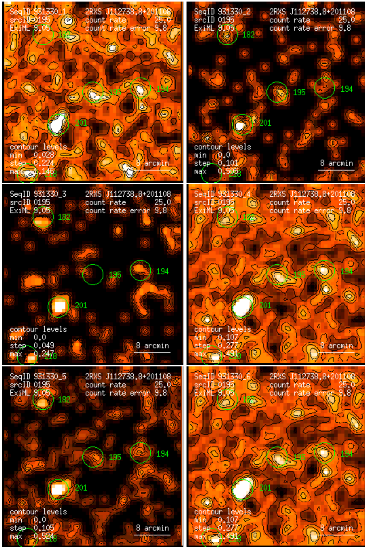
Figure 195: RASS 931330: detection 0195: band rate images, Gaussian filter: (1) PSPC channels 11 – 41, (2) 52 – 90, (3) 91 – 201, (4) 11 – 235, (5) 52 – 201, (6) 11 – 201. Broad band rates in counts/ks. Band rate contour levels in counts/ks/arcmin 2 .
