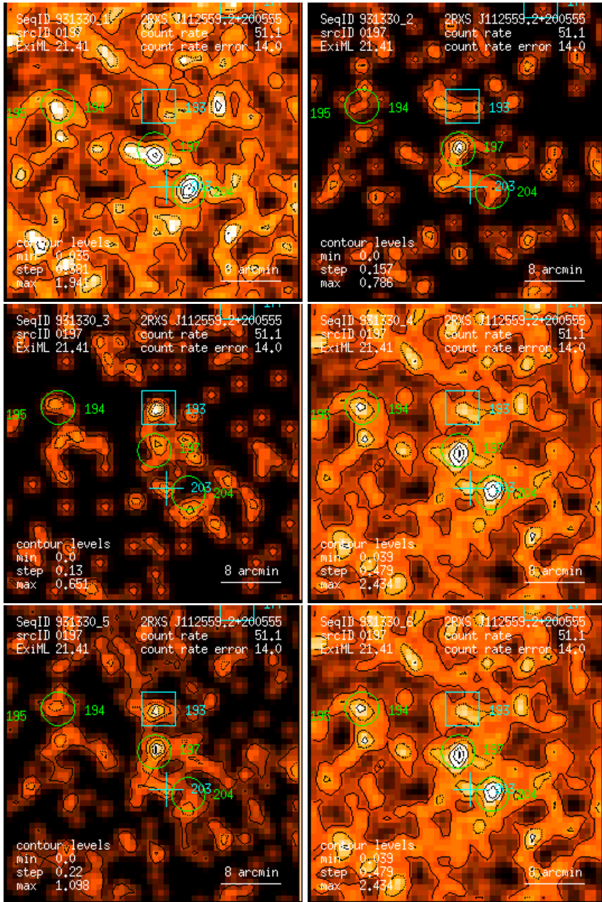
Figure 197: RASS 931330: detection 0197: band rate images, Gaussian filter: (1) PSPC channels 11 – 41, (2) 52 – 90, (3) 91 – 201, (4) 11 – 235, (5) 52 – 201, (6) 11 – 201. Broad band rates in counts/ks. Band rate contour levels in counts/ks/arcmin 2 .
