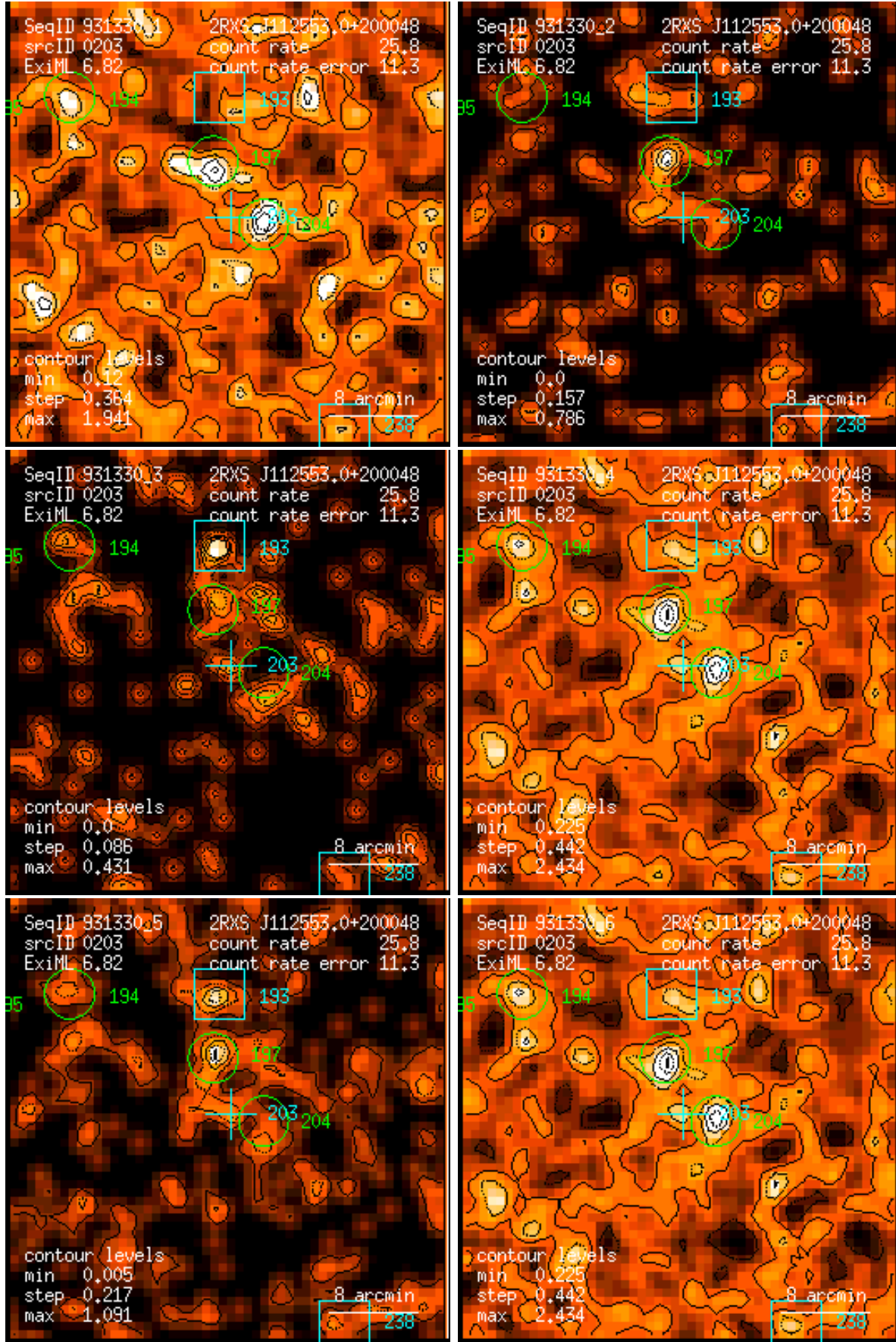
Figure 203: RASS 931330: detection 0203: band rate images, Gaussian filter: (1) PSPC channels 11 – 41, (2) 52 – 90, (3) 91 – 201, (4) 11 – 235, (5) 52 – 201, (6) 11 – 201. Broad band rates in counts/ks. Band rate contour levels in counts/ks/arcmin 2 .
