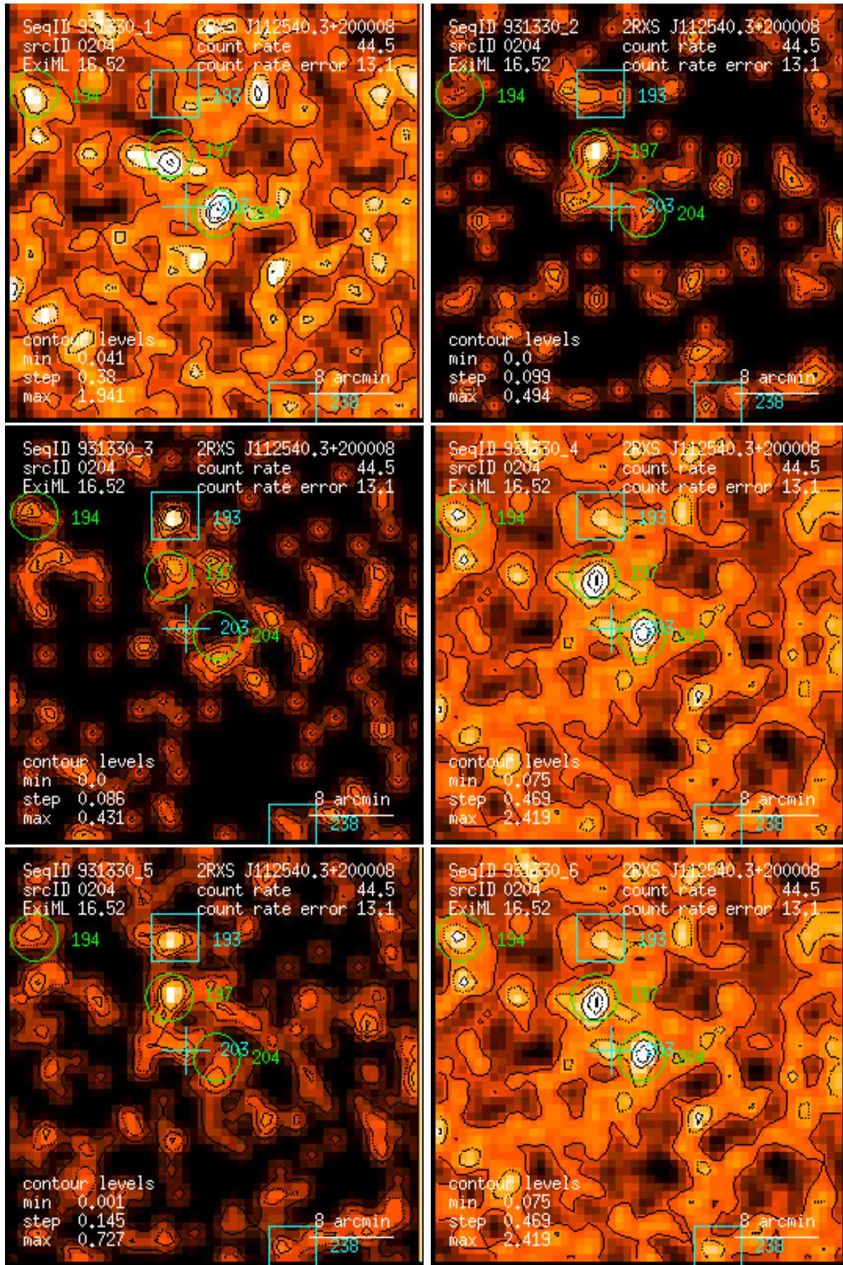
Figure 204: RASS 931330: detection 0204: band rate images, Gaussian filter: (1) PSPC channels 11 – 41, (2) 52 – 90, (3) 91 – 201, (4) 11 – 235, (5) 52 – 201, (6) 11 – 201. Broad band rates in counts/ks. Band rate contour levels in counts/ks/arcmin 2 .
