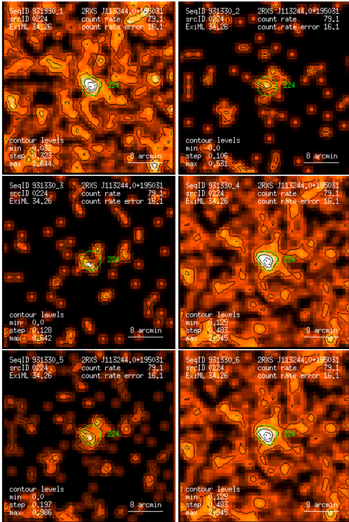
Figure 224: RASS 931330: detection 0224: band rate images, Gaussian filter: (1) PSPC channels 11 – 41, (2) 52 – 90, (3) 91 – 201, (4) 11 – 235, (5) 52 – 201, (6) 11 – 201. Broad band rates in counts/ks. Band rate contour levels in counts/ks/arcmin 2 .
