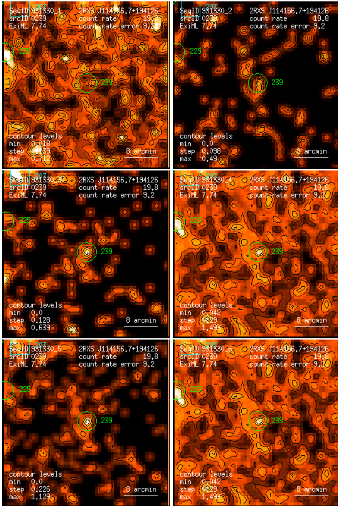
Figure 239: RASS 931330: detection 0239: band rate images, Gaussian filter: (1) PSPC channels 11 – 41, (2) 52 – 90, (3) 91 – 201, (4) 11 – 235, (5) 52 – 201, (6) 11 – 201. Broad band rates in counts/ks. Band rate contour levels in counts/ks/arcmin 2 .
