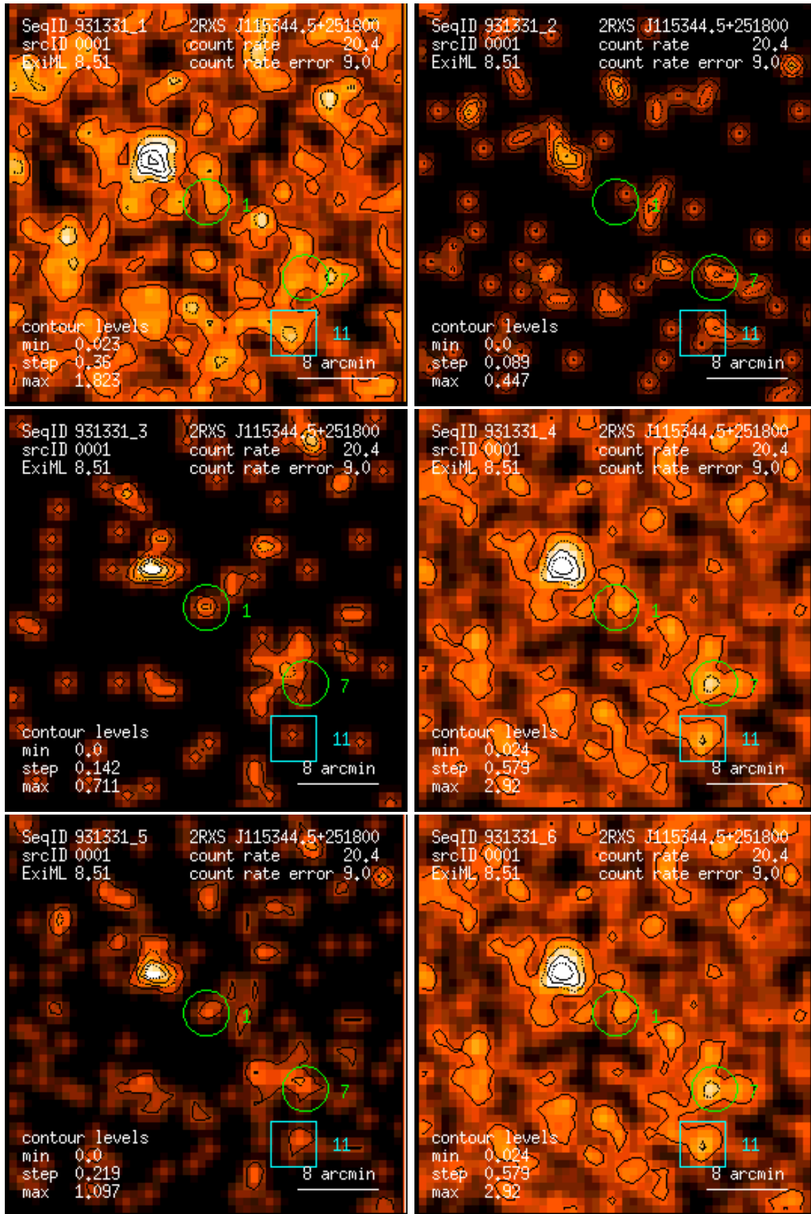
Figure 1: RASS 931331: detection 0001: band rate images, Gaussian filter: (1) PSPC channels 11 – 41, (2) 52 – 90, (3) 91 – 201, (4) 11 – 235, (5) 52 – 201, (6) 11 – 201. Broad band rates in counts/ks. Band rate contour levels in counts/ks/arcmin 2 .
