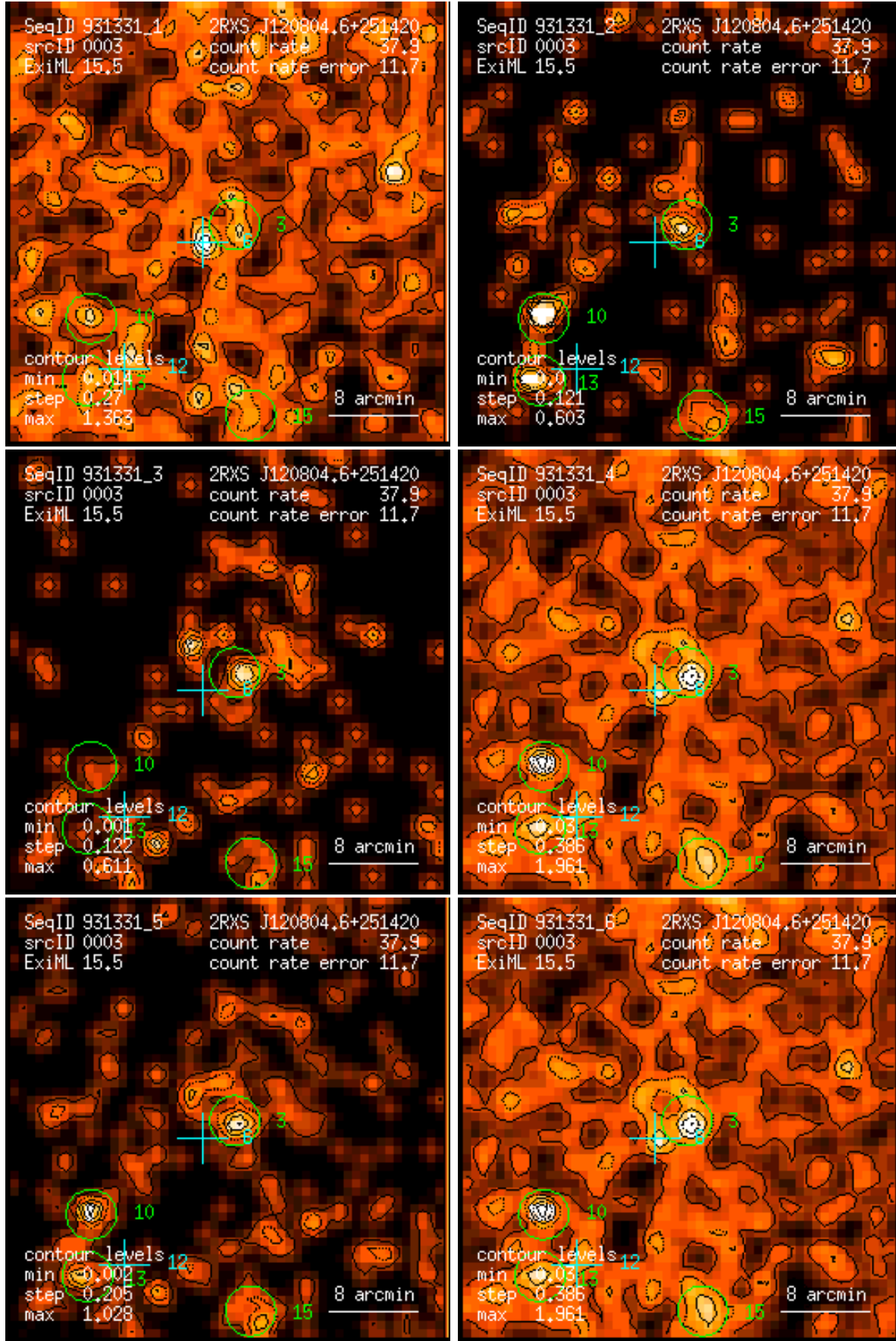
Figure 3: RASS 931331: detection 0003: band rate images, Gaussian filter: (1) PSPC channels 11 – 41, (2) 52 – 90, (3) 91 – 201, (4) 11 – 235, (5) 52 – 201, (6) 11 – 201. Broad band rates in counts/ks. Band rate contour levels in counts/ks/arcmin 2 .
