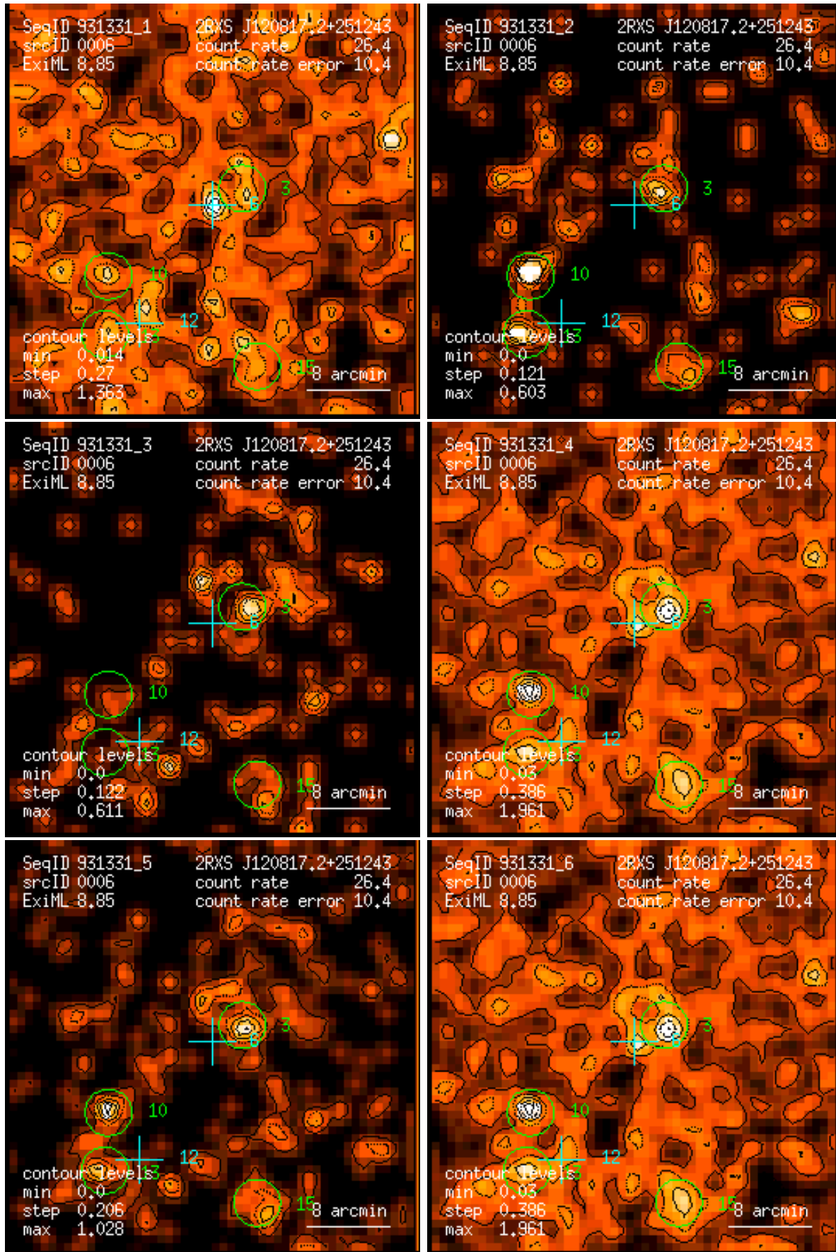
Figure 6: RASS 931331: detection 0006: band rate images, Gaussian filter: (1) PSPC channels 11 – 41, (2) 52 – 90, (3) 91 – 201, (4) 11 – 235, (5) 52 – 201, (6) 11 – 201. Broad band rates in counts/ks. Band rate contour levels in counts/ks/arcmin 2 .
