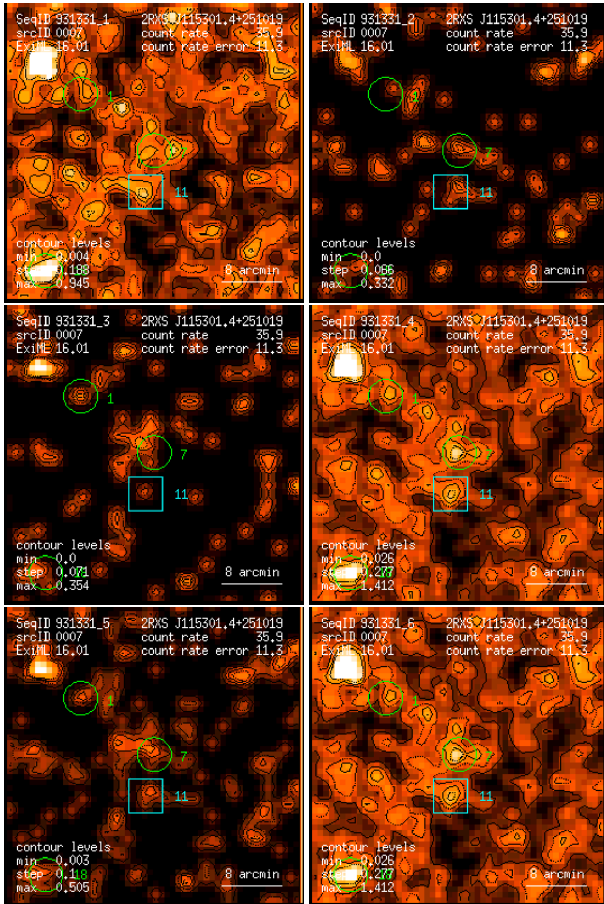
Figure 7: RASS 931331: detection 0007: band rate images, Gaussian filter: (1) PSPC channels 11 – 41, (2) 52 – 90, (3) 91 – 201, (4) 11 – 235, (5) 52 – 201, (6) 11 – 201. Broad band rates in counts/ks. Band rate contour levels in counts/ks/arcmin 2 .
