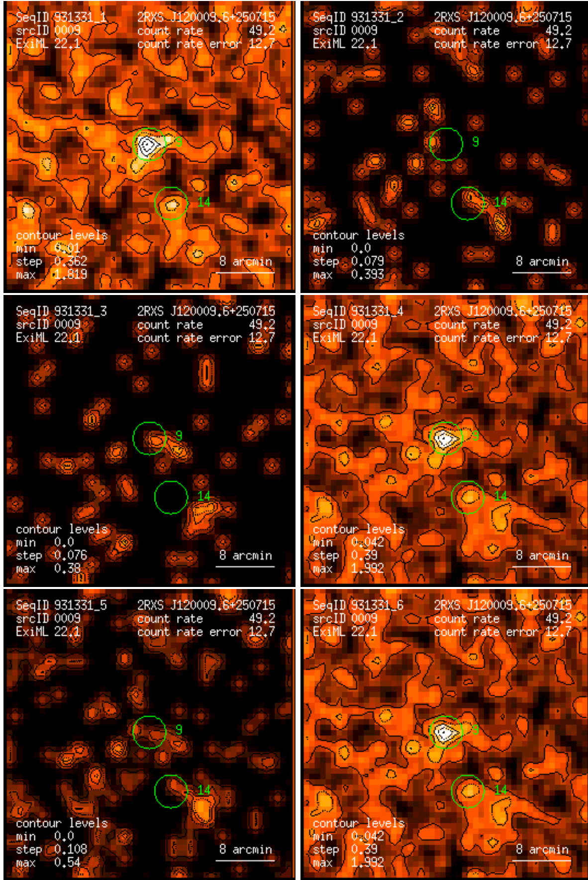
Figure 9: RASS 931331: detection 0009: band rate images, Gaussian filter: (1) PSPC channels 11 – 41, (2) 52 – 90, (3) 91 – 201, (4) 11 – 235, (5) 52 – 201, (6) 11 – 201. Broad band rates in counts/ks. Band rate contour levels in counts/ks/arcmin 2 .
