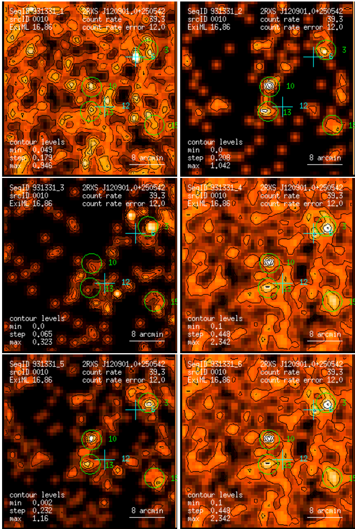
Figure 10: RASS 931331: detection 0010: band rate images, Gaussian filter: (1) PSPC channels 11 – 41, (2) 52 – 90, (3) 91 – 201, (4) 11 – 235, (5) 52 – 201, (6) 11 – 201. Broad band rates in counts/ks. Band rate contour levels in counts/ks/arcmin 2 .
