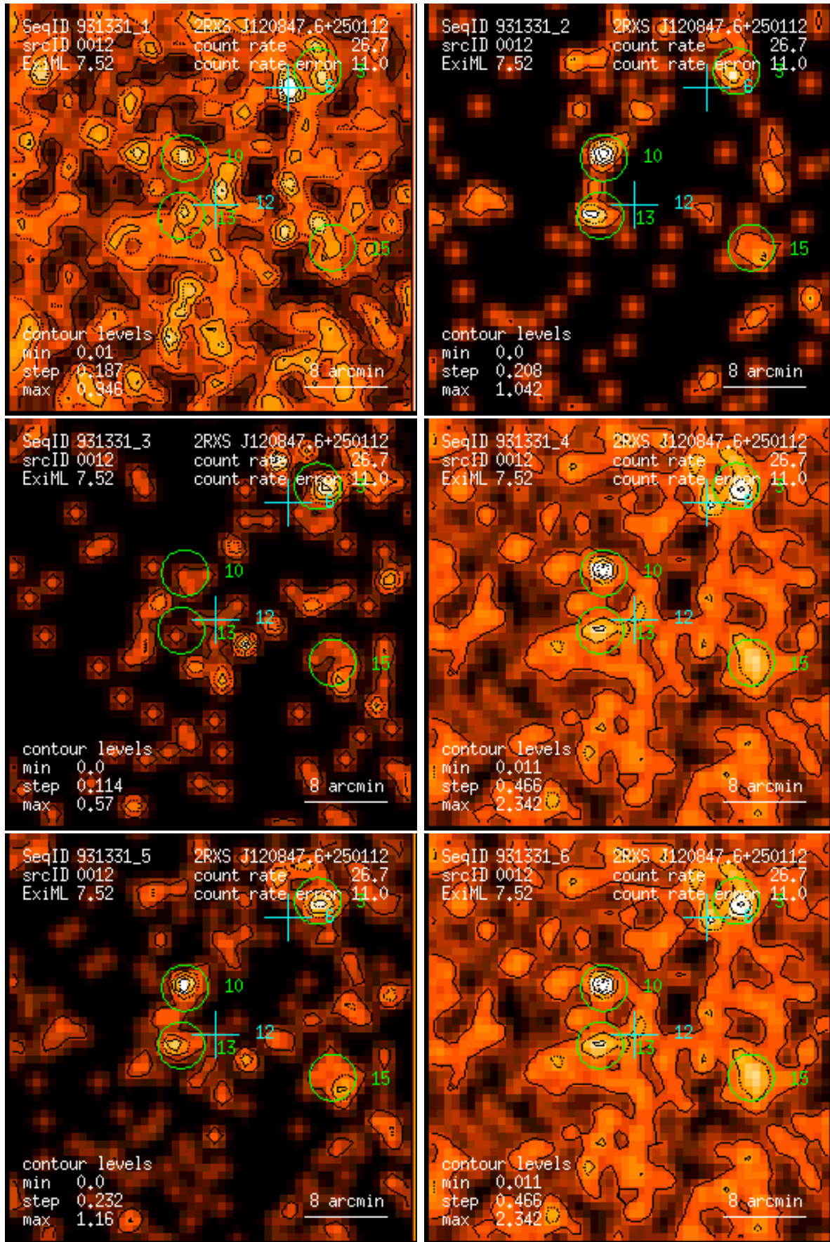
Figure 12: RASS 931331: detection 0012: band rate images, Gaussian filter: (1) PSPC channels 11 – 41, (2) 52 – 90, (3) 91 – 201, (4) 11 – 235, (5) 52 – 201, (6) 11 – 201. Broad band rates in counts/ks. Band rate contour levels in counts/ks/arcmin 2 .
