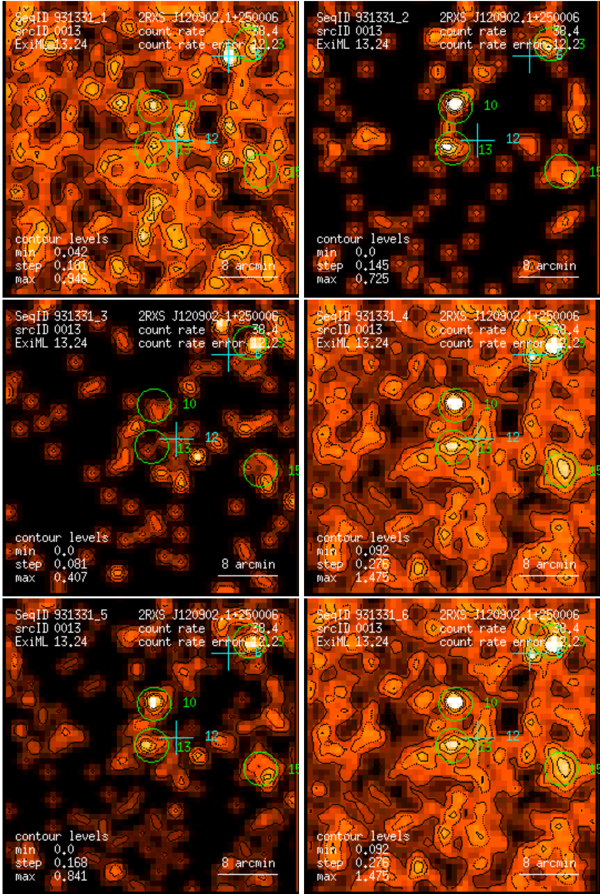
Figure 13: RASS 931331: detection 0013: band rate images, Gaussian filter: (1) PSPC channels 11 – 41, (2) 52 – 90, (3) 91 – 201, (4) 11 – 235, (5) 52 – 201, (6) 11 – 201. Broad band rates in counts/ks. Band rate contour levels in counts/ks/arcmin 2 .
