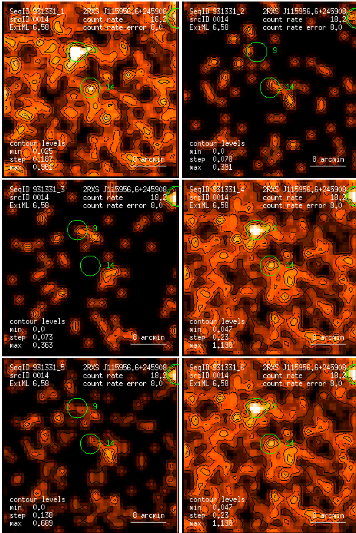
Figure 14: RASS 931331: detection 0014: band rate images, Gaussian filter: (1) PSPC channels 11 – 41, (2) 52 – 90, (3) 91 – 201, (4) 11 – 235, (5) 52 – 201, (6) 11 – 201. Broad band rates in counts/ks. Band rate contour levels in counts/ks/arcmin 2 .
