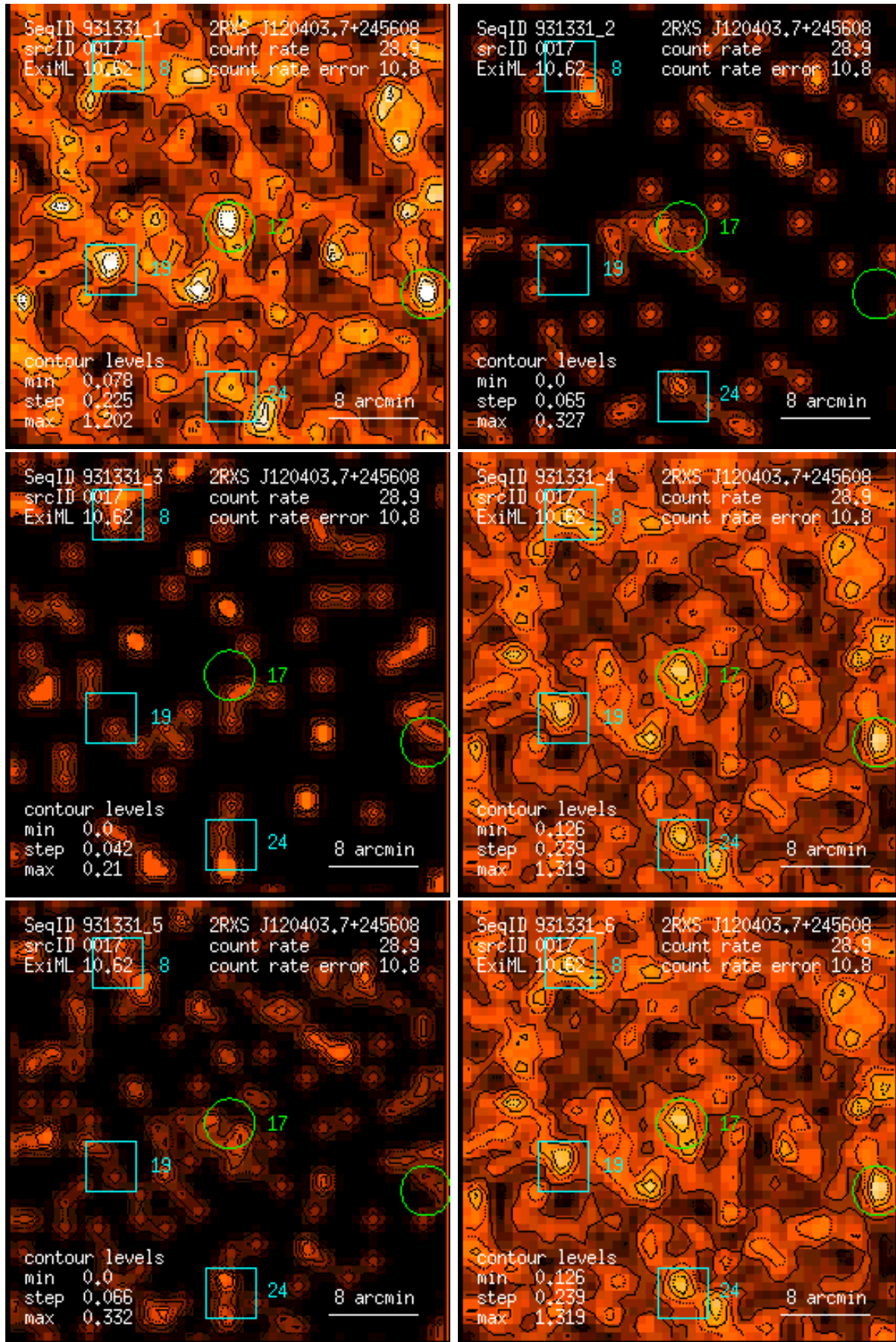
Figure 17: RASS 931331: detection 0017: band rate images, Gaussian filter: (1) PSPC channels 11 – 41, (2) 52 – 90, (3) 91 – 201, (4) 11 – 235, (5) 52 – 201, (6) 11 – 201. Broad band rates in counts/ks. Band rate contour levels in counts/ks/arcmin 2 .
