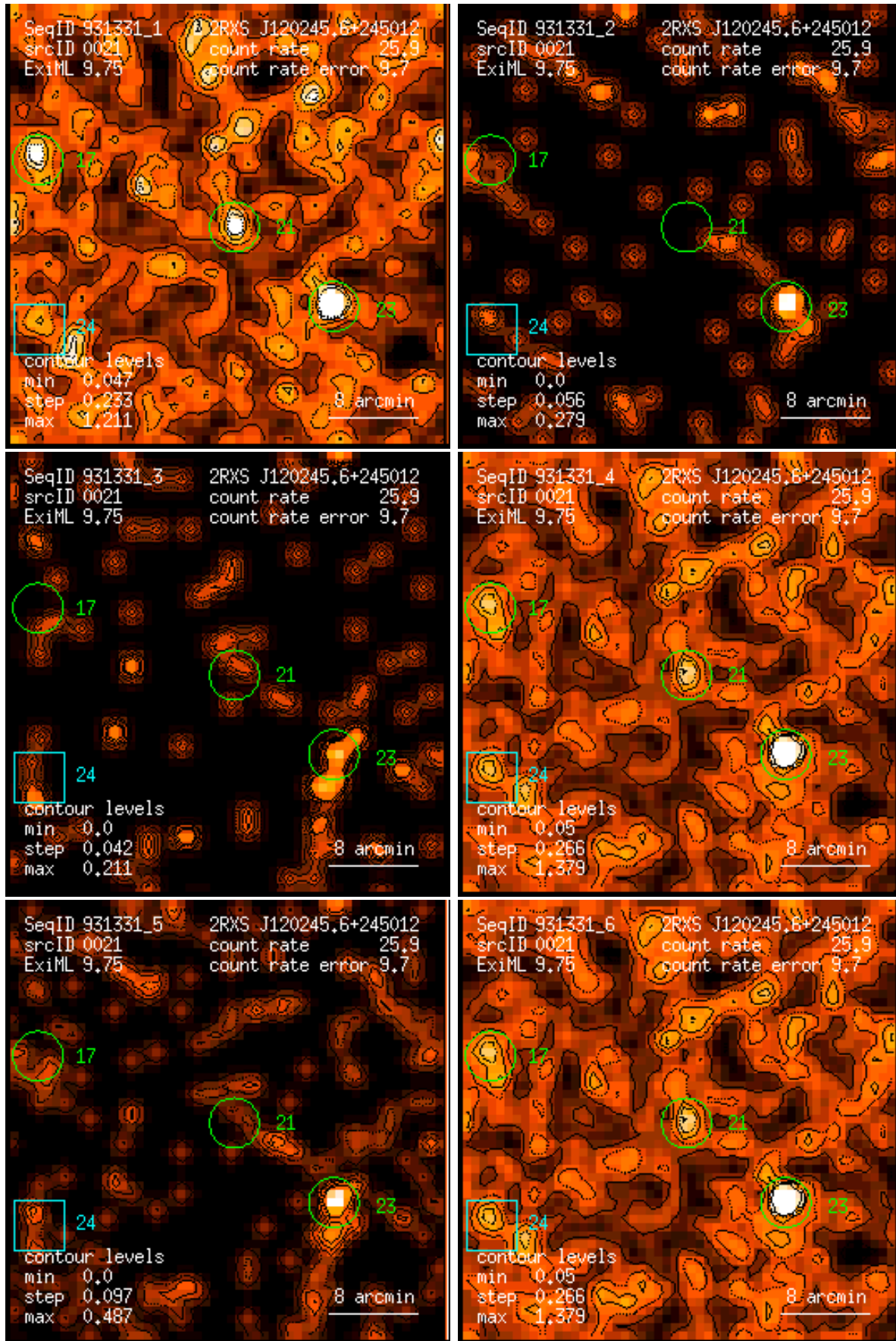
Figure 21: RASS 931331: detection 0021: band rate images, Gaussian filter: (1) PSPC channels 11 – 41, (2) 52 – 90, (3) 91 – 201, (4) 11 – 235, (5) 52 – 201, (6) 11 – 201. Broad band rates in counts/ks. Band rate contour levels in counts/ks/arcmin 2 .
