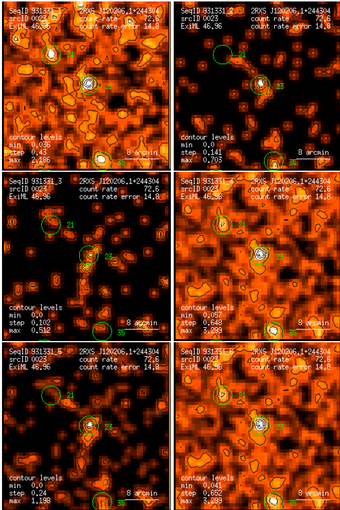
Figure 23: RASS 931331: detection 0023: band rate images, Gaussian filter: (1) PSPC channels 11 – 41, (2) 52 – 90, (3) 91 – 201, (4) 11 – 235, (5) 52 – 201, (6) 11 – 201. Broad band rates in counts/ks. Band rate contour levels in counts/ks/arcmin 2 .
