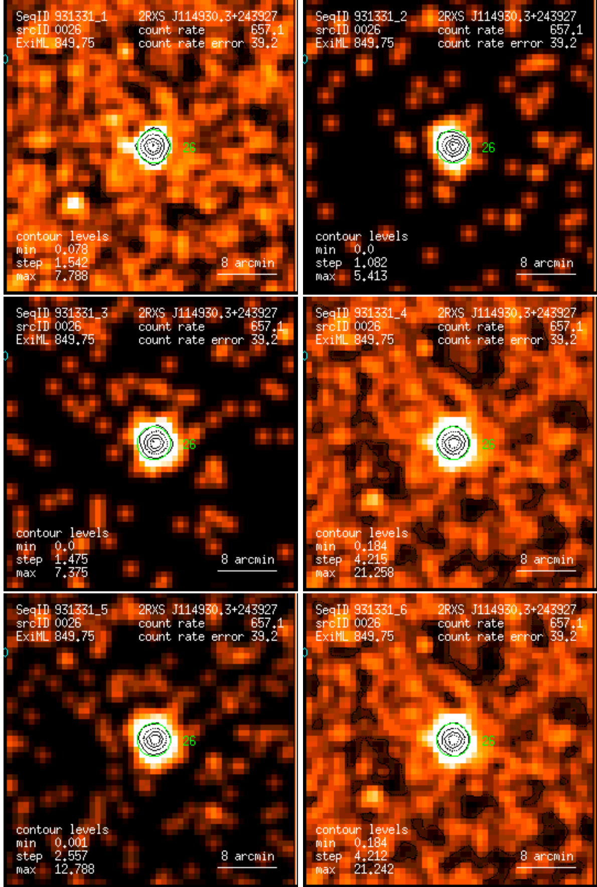
Figure 26: RASS 931331: detection 0026: band rate images, Gaussian filter: (1) PSPC channels 11 – 41, (2) 52 – 90, (3) 91 – 201, (4) 11 – 235, (5) 52 – 201, (6) 11 – 201. Broad band rates in counts/ks. Band rate contour levels in counts/ks/arcmin 2 .
