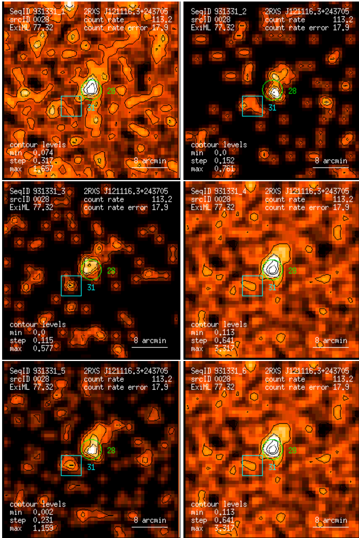
Figure 28: RASS 931331: detection 0028: band rate images, Gaussian filter: (1) PSPC channels 11 – 41, (2) 52 – 90, (3) 91 – 201, (4) 11 – 235, (5) 52 – 201, (6) 11 – 201. Broad band rates in counts/ks. Band rate contour levels in counts/ks/arcmin 2 .
