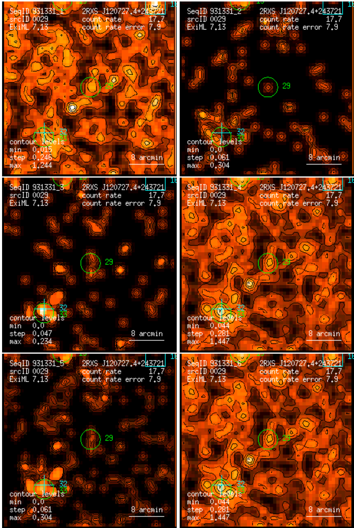
Figure 29: RASS 931331: detection 0029: band rate images, Gaussian filter: (1) PSPC channels 11 – 41, (2) 52 – 90, (3) 91 – 201, (4) 11 – 235, (5) 52 – 201, (6) 11 – 201. Broad band rates in counts/ks. Band rate contour levels in counts/ks/arcmin 2 .
