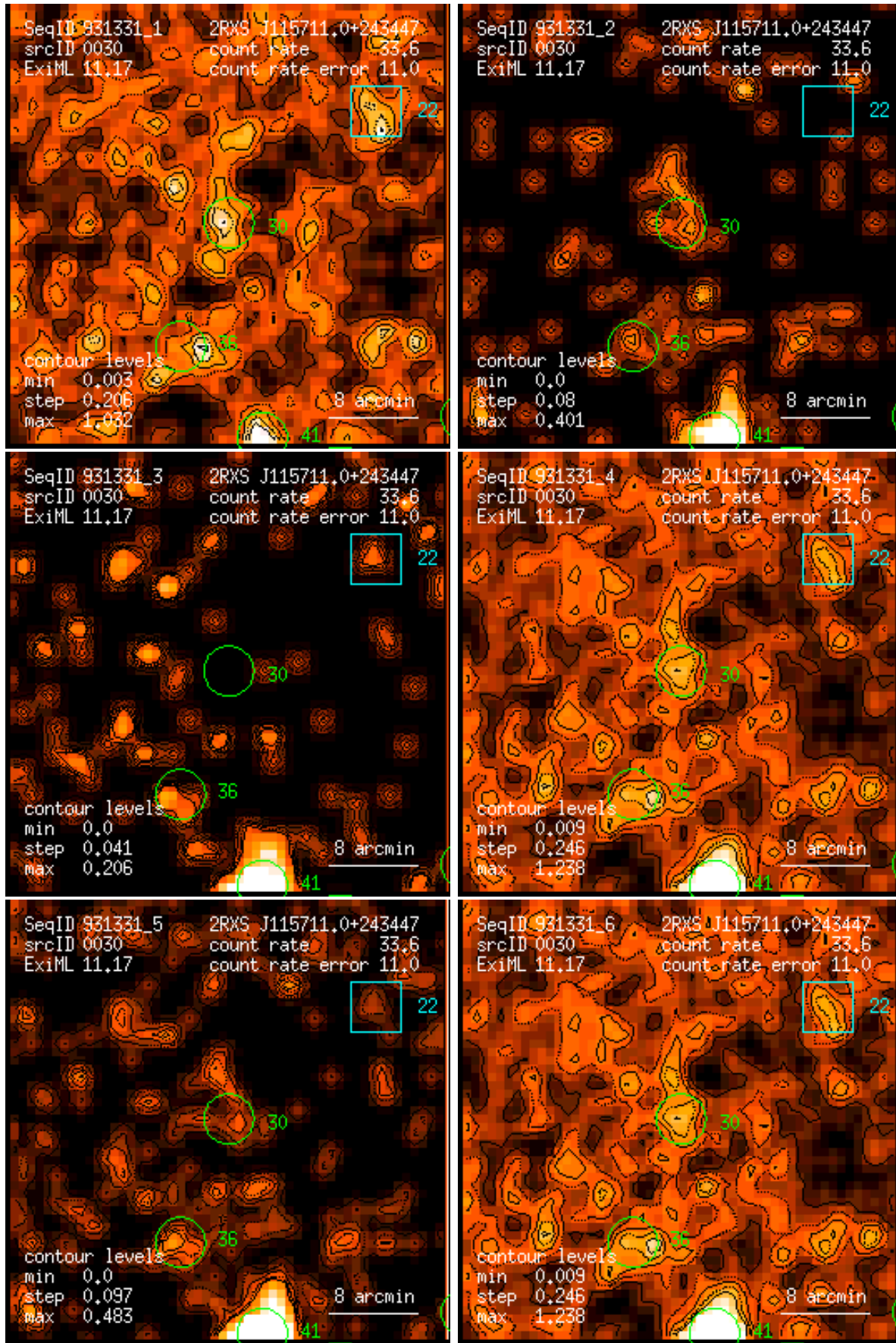
Figure 30: RASS 931331: detection 0030: band rate images, Gaussian filter: (1) PSPC channels 11 – 41, (2) 52 – 90, (3) 91 – 201, (4) 11 – 235, (5) 52 – 201, (6) 11 – 201. Broad band rates in counts/ks. Band rate contour levels in counts/ks/arcmin 2 .
