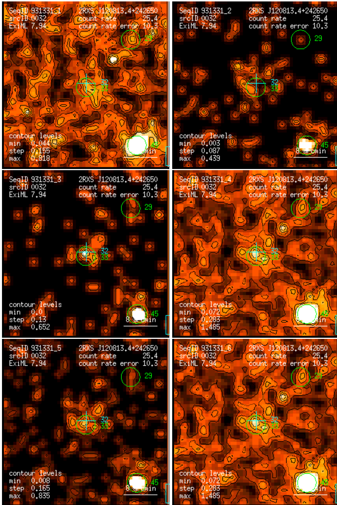
Figure 32: RASS 931331: detection 0032: band rate images, Gaussian filter: (1) PSPC channels 11 – 41, (2) 52 – 90, (3) 91 – 201, (4) 11 – 235, (5) 52 – 201, (6) 11 – 201. Broad band rates in counts/ks. Band rate contour levels in counts/ks/arcmin 2 .
