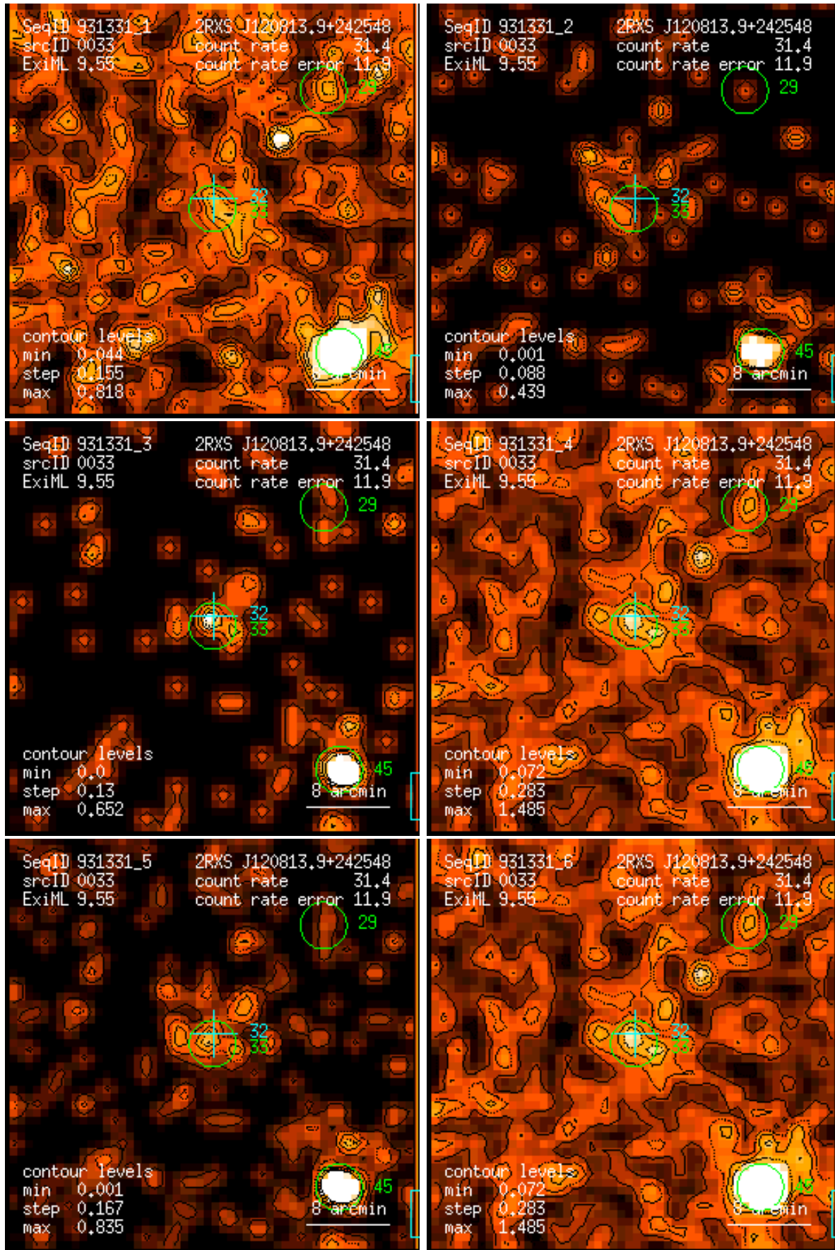
Figure 33: RASS 931331: detection 0033: band rate images, Gaussian filter: (1) PSPC channels 11 – 41, (2) 52 – 90, (3) 91 – 201, (4) 11 – 235, (5) 52 – 201, (6) 11 – 201. Broad band rates in counts/ks. Band rate contour levels in counts/ks/arcmin 2 .
