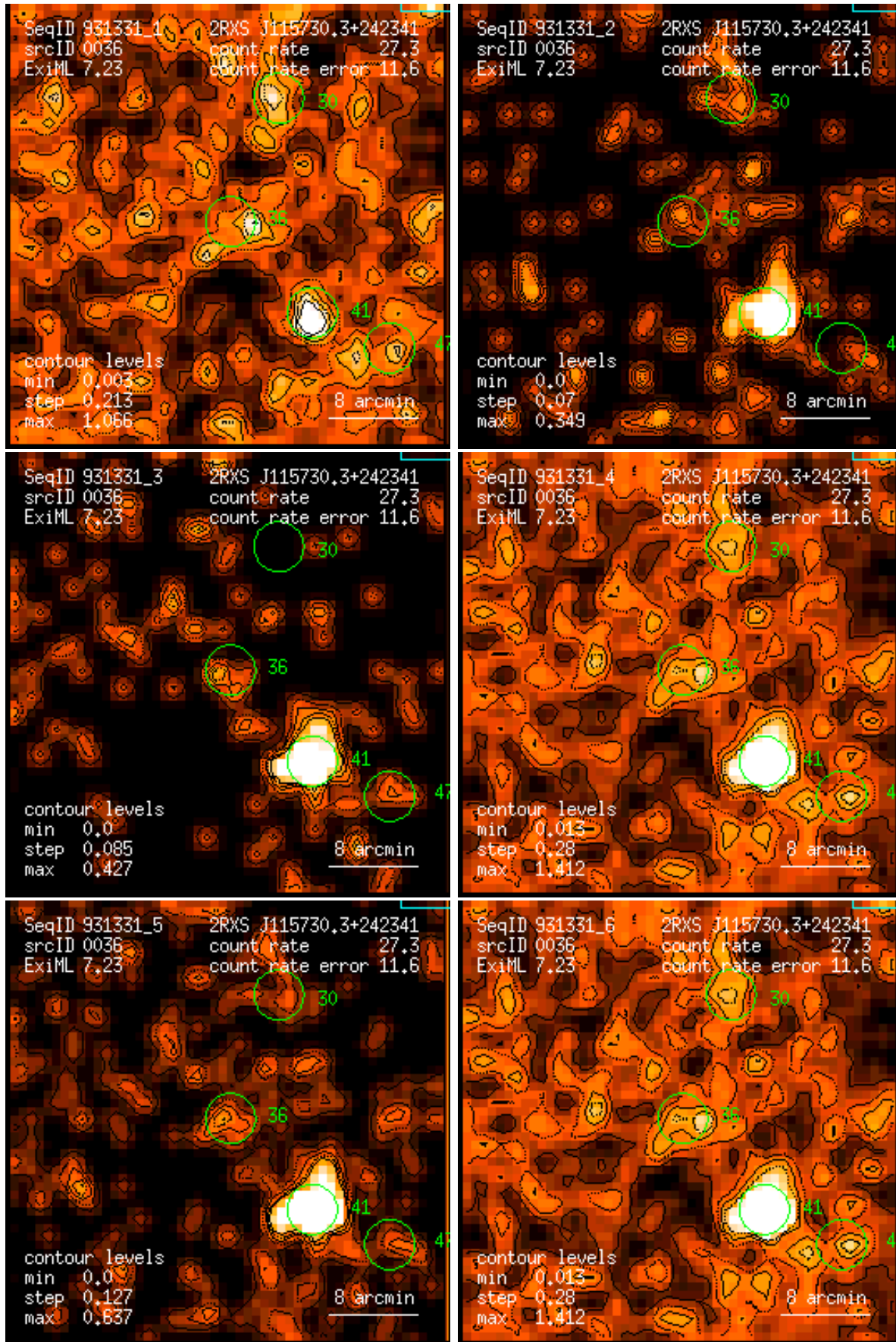
Figure 36: RASS 931331: detection 0036: band rate images, Gaussian filter: (1) PSPC channels 11 – 41, (2) 52 – 90, (3) 91 – 201, (4) 11 – 235, (5) 52 – 201, (6) 11 – 201. Broad band rates in counts/ks. Band rate contour levels in counts/ks/arcmin 2 .
