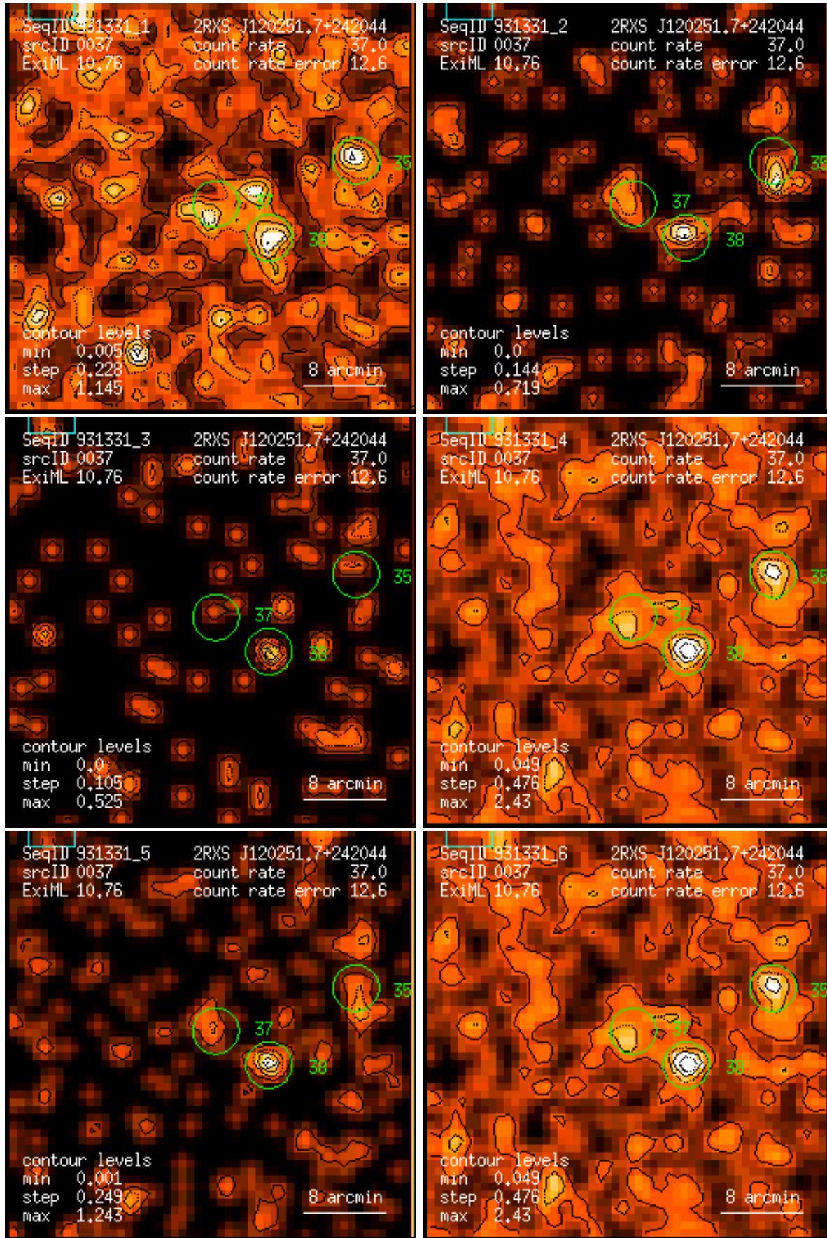
Figure 37: RASS 931331: detection 0037: band rate images, Gaussian filter: (1) PSPC channels 11 – 41, (2) 52 – 90, (3) 91 – 201, (4) 11 – 235, (5) 52 – 201, (6) 11 – 201. Broad band rates in counts/ks. Band rate contour levels in counts/ks/arcmin 2 .
