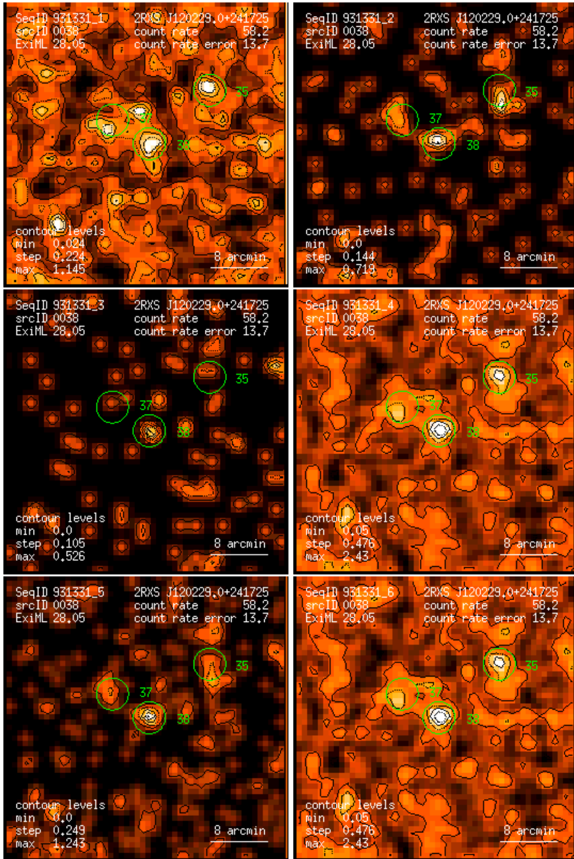
Figure 38: RASS 931331: detection 0038: band rate images, Gaussian filter: (1) PSPC channels 11 – 41, (2) 52 – 90, (3) 91 – 201, (4) 11 – 235, (5) 52 – 201, (6) 11 – 201. Broad band rates in counts/ks. Band rate contour levels in counts/ks/arcmin 2 .
