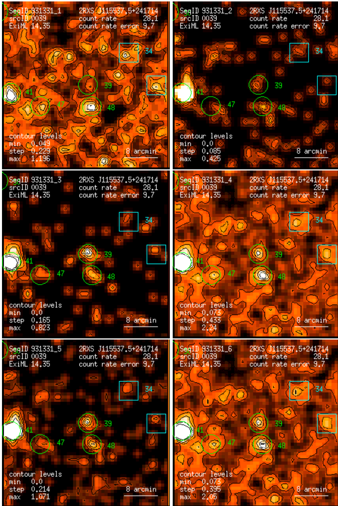
Figure 39: RASS 931331: detection 0039: band rate images, Gaussian filter: (1) PSPC channels 11 – 41, (2) 52 – 90, (3) 91 – 201, (4) 11 – 235, (5) 52 – 201, (6) 11 – 201. Broad band rates in counts/ks. Band rate contour levels in counts/ks/arcmin 2 .
