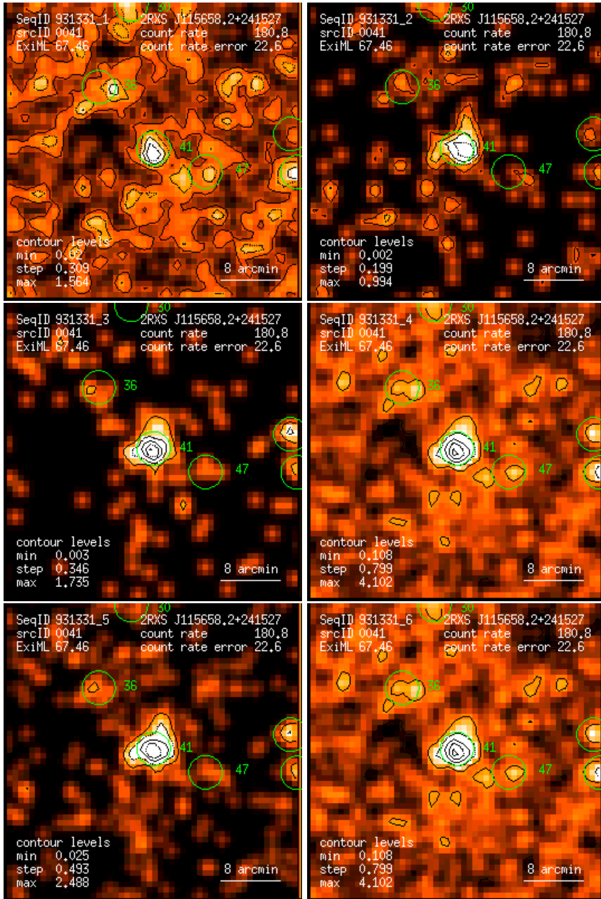
Figure 41: RASS 931331: detection 0041: band rate images, Gaussian filter: (1) PSPC channels 11 – 41, (2) 52 – 90, (3) 91 – 201, (4) 11 – 235, (5) 52 – 201, (6) 11 – 201. Broad band rates in counts/ks. Band rate contour levels in counts/ks/arcmin 2 .
