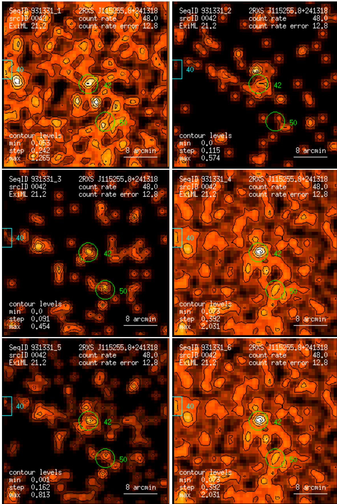
Figure 42: RASS 931331: detection 0042: band rate images, Gaussian filter: (1) PSPC channels 11 – 41, (2) 52 – 90, (3) 91 – 201, (4) 11 – 235, (5) 52 – 201, (6) 11 – 201. Broad band rates in counts/ks. Band rate contour levels in counts/ks/arcmin 2 .
