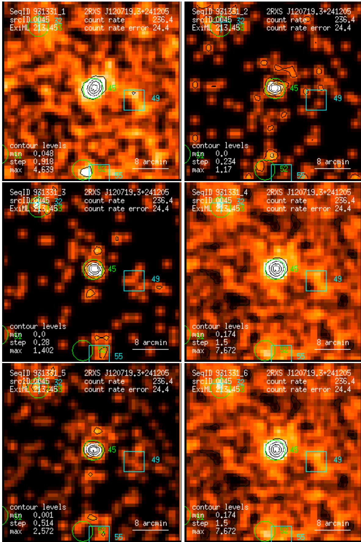
Figure 45: RASS 931331: detection 0045: band rate images, Gaussian filter: (1) PSPC channels 11 – 41, (2) 52 – 90, (3) 91 – 201, (4) 11 – 235, (5) 52 – 201, (6) 11 – 201. Broad band rates in counts/ks. Band rate contour levels in counts/ks/arcmin 2 .
