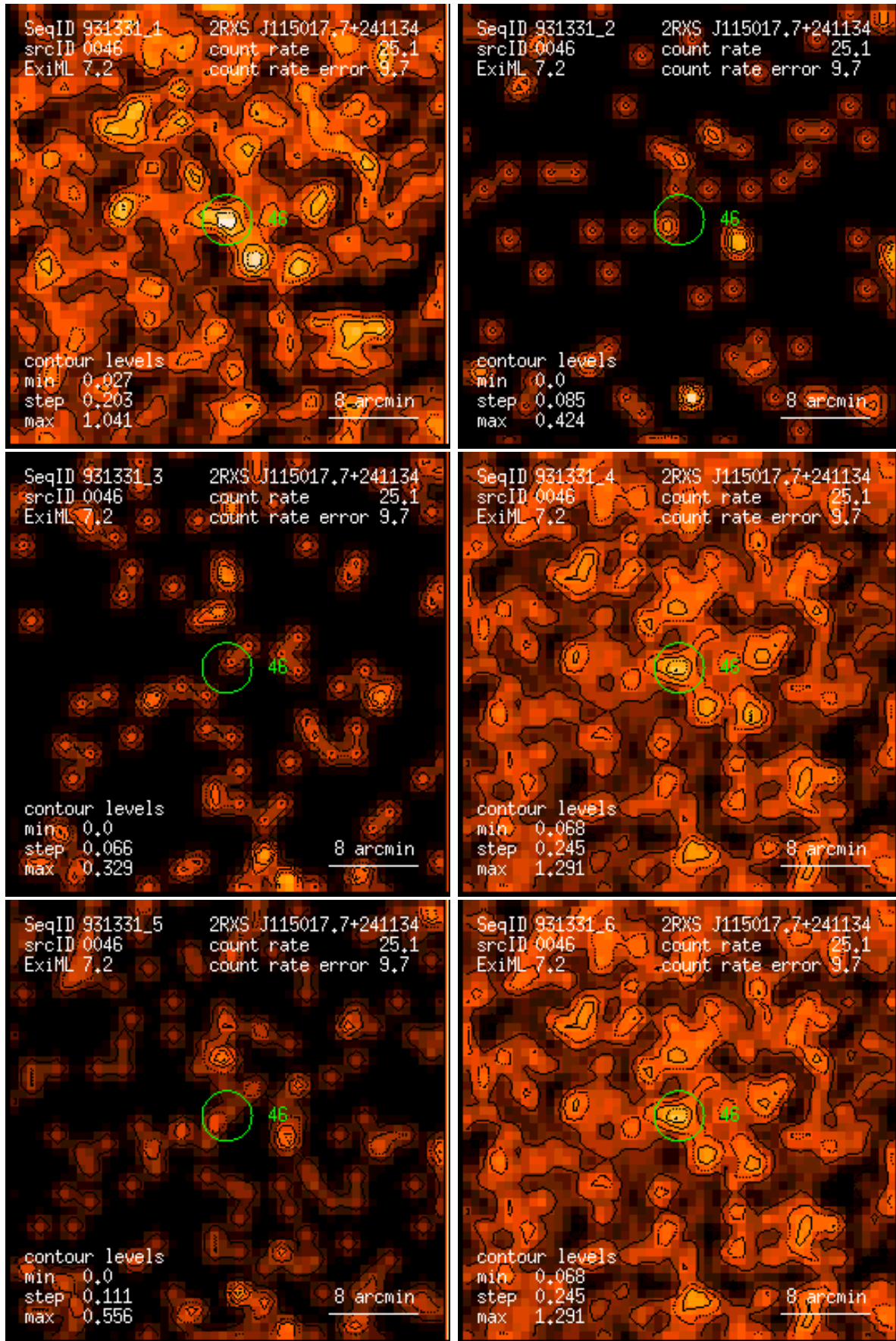
Figure 46: RASS 931331: detection 0046: band rate images, Gaussian filter: (1) PSPC channels 11 – 41, (2) 52 – 90, (3) 91 – 201, (4) 11 – 235, (5) 52 – 201, (6) 11 – 201. Broad band rates in counts/ks. Band rate contour levels in counts/ks/arcmin 2 .
