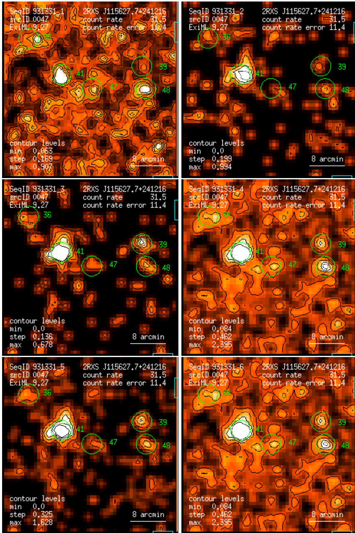
Figure 47: RASS 931331: detection 0047: band rate images, Gaussian filter: (1) PSPC channels 11 – 41, (2) 52 – 90, (3) 91 – 201, (4) 11 – 235, (5) 52 – 201, (6) 11 – 201. Broad band rates in counts/ks. Band rate contour levels in counts/ks/arcmin 2 .
