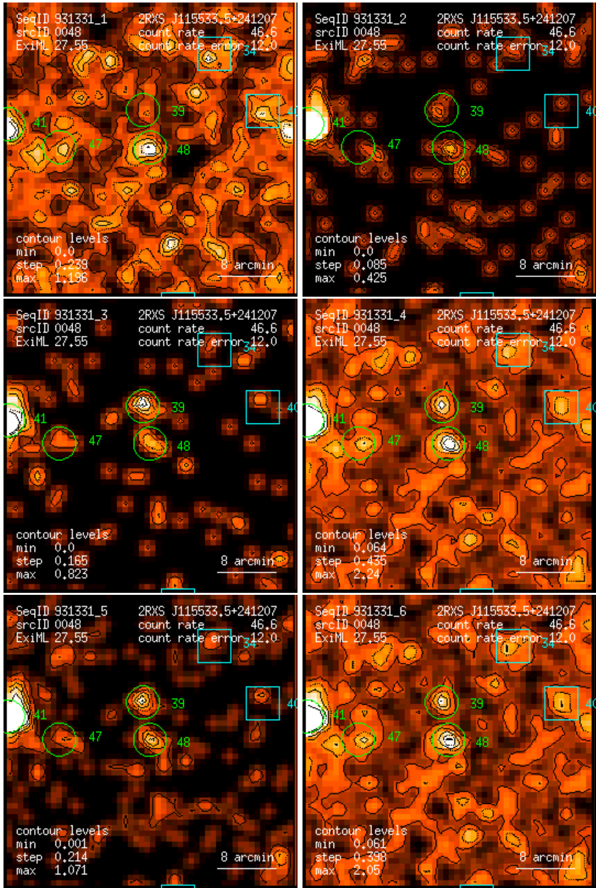
Figure 48: RASS 931331: detection 0048: band rate images, Gaussian filter: (1) PSPC channels 11 – 41, (2) 52 – 90, (3) 91 – 201, (4) 11 – 235, (5) 52 – 201, (6) 11 – 201. Broad band rates in counts/ks. Band rate contour levels in counts/ks/arcmin 2 .
