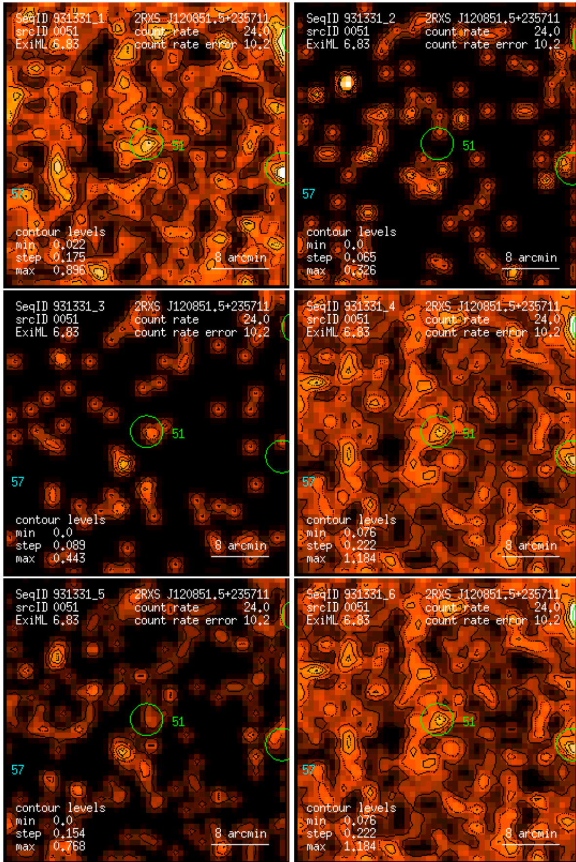
Figure 51: RASS 931331: detection 0051: band rate images, Gaussian filter: (1) PSPC channels 11 – 41, (2) 52 – 90, (3) 91 – 201, (4) 11 – 235, (5) 52 – 201, (6) 11 – 201. Broad band rates in counts/ks. Band rate contour levels in counts/ks/arcmin 2 .
