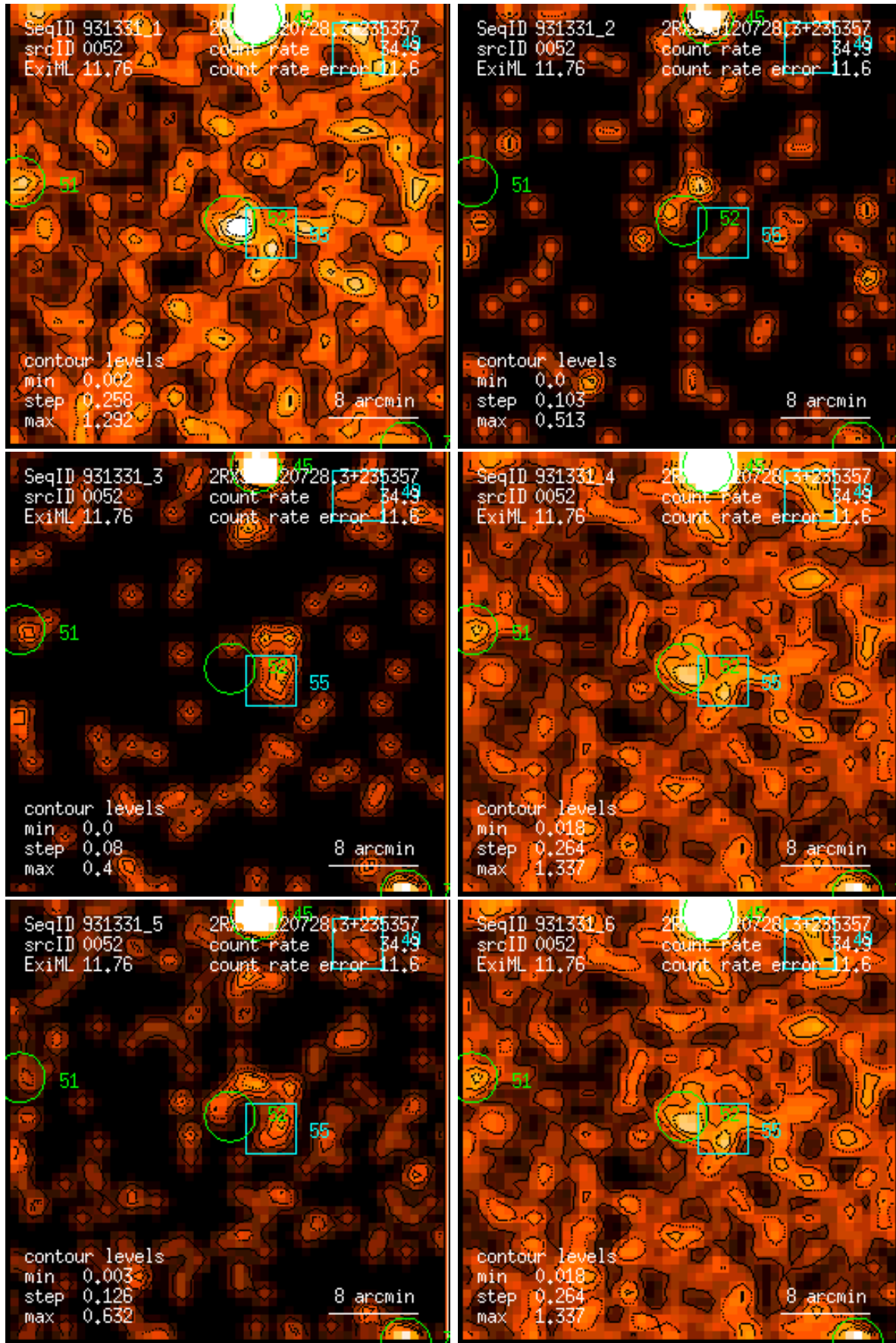
Figure 52: RASS 931331: detection 0052: band rate images, Gaussian filter: (1) PSPC channels 11 – 41, (2) 52 – 90, (3) 91 – 201, (4) 11 – 235, (5) 52 – 201, (6) 11 – 201. Broad band rates in counts/ks. Band rate contour levels in counts/ks/arcmin 2 .
