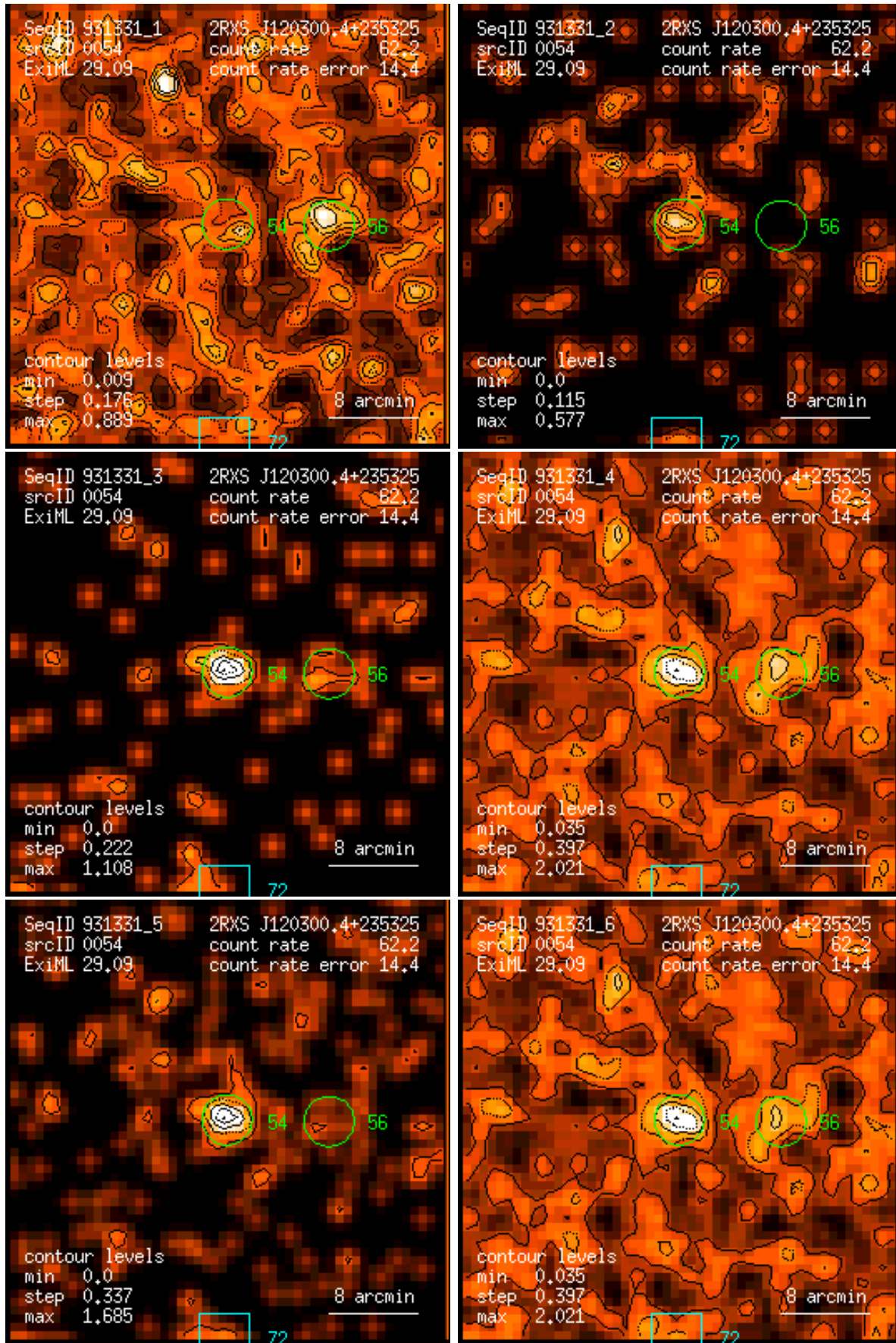
Figure 54: RASS 931331: detection 0054: band rate images, Gaussian filter: (1) PSPC channels 11 – 41, (2) 52 – 90, (3) 91 – 201, (4) 11 – 235, (5) 52 – 201, (6) 11 – 201. Broad band rates in counts/ks. Band rate contour levels in counts/ks/arcmin 2 .
