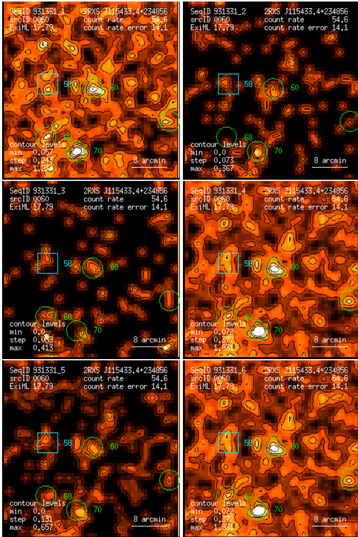
Figure 60: RASS 931331: detection 0060: band rate images, Gaussian filter: (1) PSPC channels 11 – 41, (2) 52 – 90, (3) 91 – 201, (4) 11 – 235, (5) 52 – 201, (6) 11 – 201. Broad band rates in counts/ks. Band rate contour levels in counts/ks/arcmin 2 .
