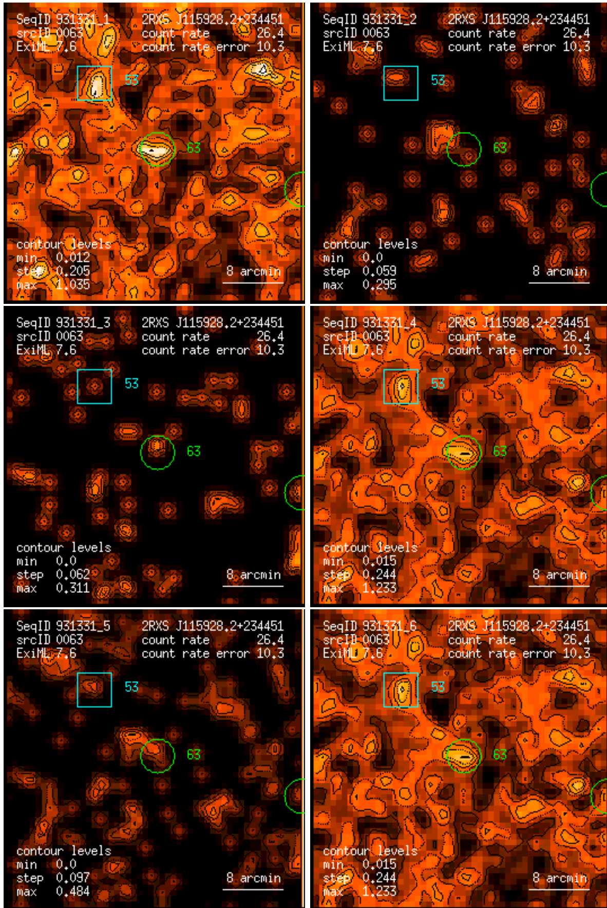
Figure 63: RASS 931331: detection 0063: band rate images, Gaussian filter: (1) PSPC channels 11 – 41, (2) 52 – 90, (3) 91 – 201, (4) 11 – 235, (5) 52 – 201, (6) 11 – 201. Broad band rates in counts/ks. Band rate contour levels in counts/ks/arcmin 2 .
