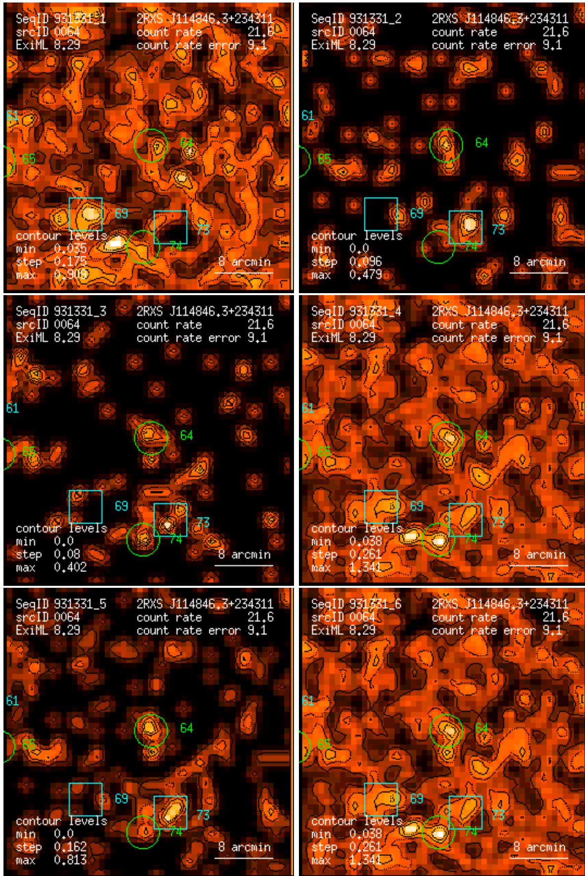
Figure 64: RASS 931331: detection 0064: band rate images, Gaussian filter: (1) PSPC channels 11 – 41, (2) 52 – 90, (3) 91 – 201, (4) 11 – 235, (5) 52 – 201, (6) 11 – 201. Broad band rates in counts/ks. Band rate contour levels in counts/ks/arcmin 2 .
