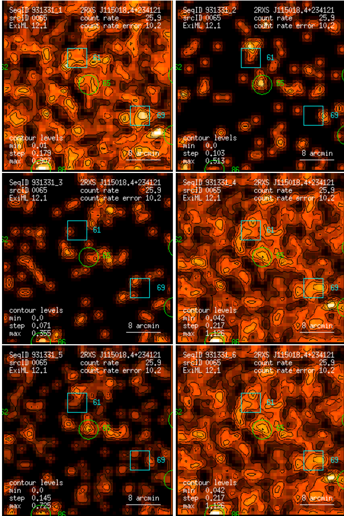
Figure 65: RASS 931331: detection 0065: band rate images, Gaussian filter: (1) PSPC channels 11 – 41, (2) 52 – 90, (3) 91 – 201, (4) 11 – 235, (5) 52 – 201, (6) 11 – 201. Broad band rates in counts/ks. Band rate contour levels in counts/ks/arcmin 2 .
