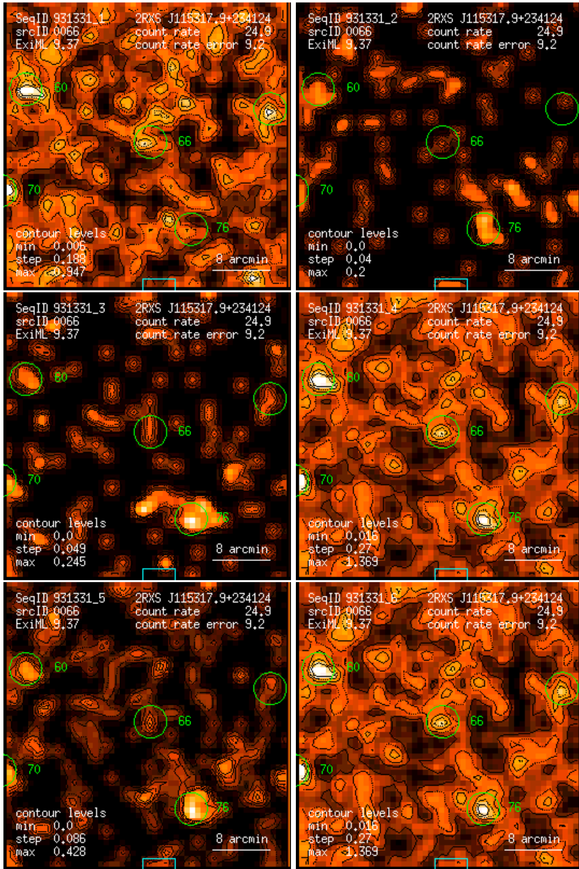
Figure 66: RASS 931331: detection 0066: band rate images, Gaussian filter: (1) PSPC channels 11 – 41, (2) 52 – 90, (3) 91 – 201, (4) 11 – 235, (5) 52 – 201, (6) 11 – 201. Broad band rates in counts/ks. Band rate contour levels in counts/ks/arcmin 2 .
