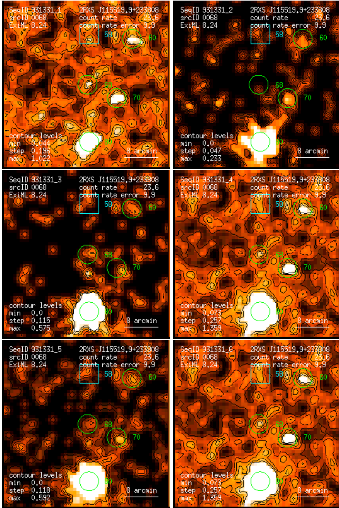
Figure 68: RASS 931331: detection 0068: band rate images, Gaussian filter: (1) PSPC channels 11 – 41, (2) 52 – 90, (3) 91 – 201, (4) 11 – 235, (5) 52 – 201, (6) 11 – 201. Broad band rates in counts/ks. Band rate contour levels in counts/ks/arcmin 2 .
