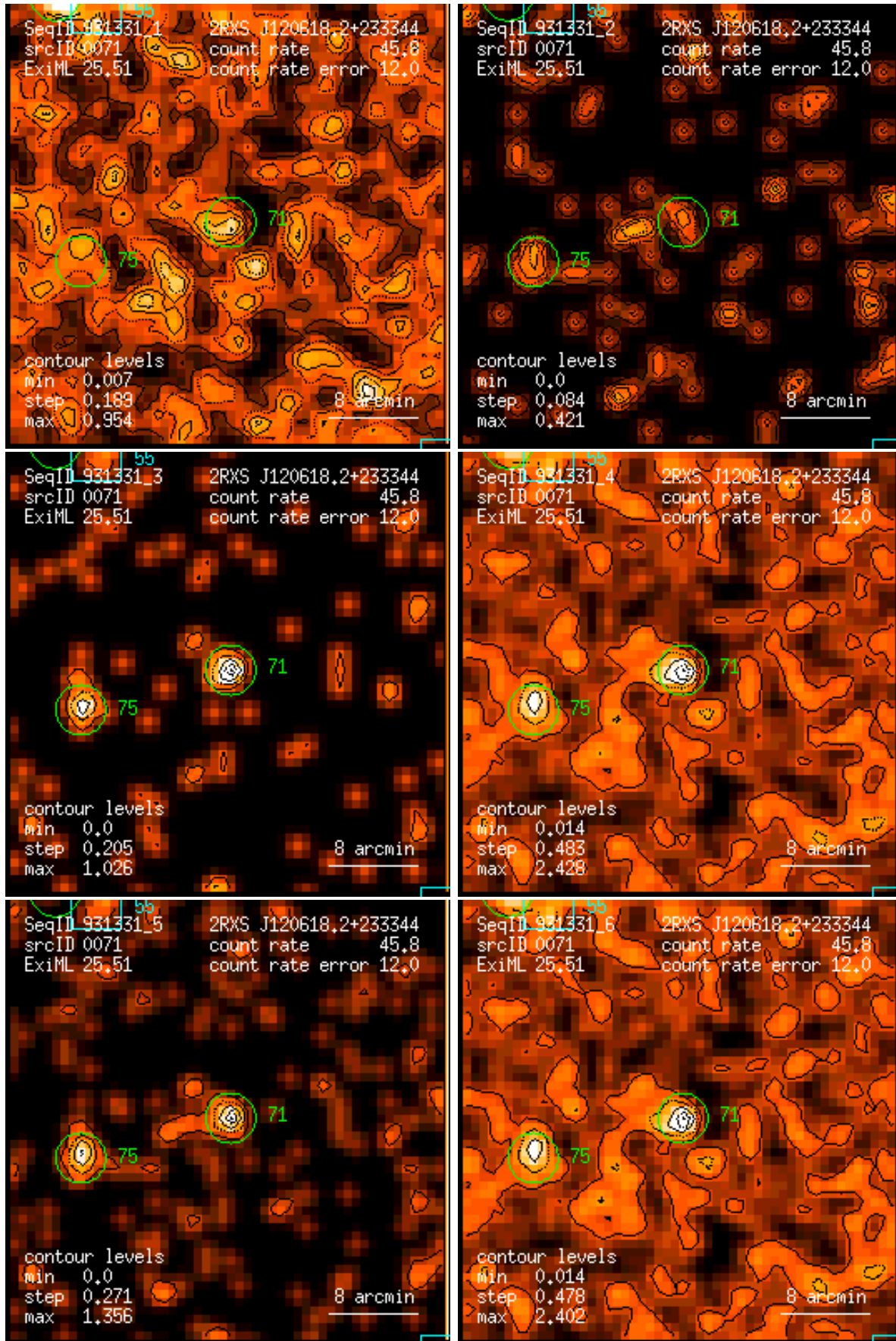
Figure 71: RASS 931331: detection 0071: band rate images, Gaussian filter: (1) PSPC channels 11 – 41, (2) 52 – 90, (3) 91 – 201, (4) 11 – 235, (5) 52 – 201, (6) 11 – 201. Broad band rates in counts/ks. Band rate contour levels in counts/ks/arcmin 2 .
