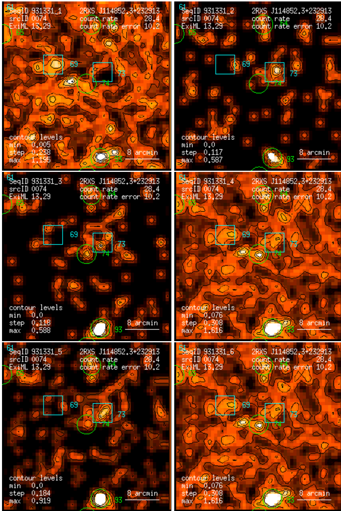
Figure 74: RASS 931331: detection 0074: band rate images, Gaussian filter: (1) PSPC channels 11 – 41, (2) 52 – 90, (3) 91 – 201, (4) 11 – 235, (5) 52 – 201, (6) 11 – 201. Broad band rates in counts/ks. Band rate contour levels in counts/ks/arcmin 2 .
