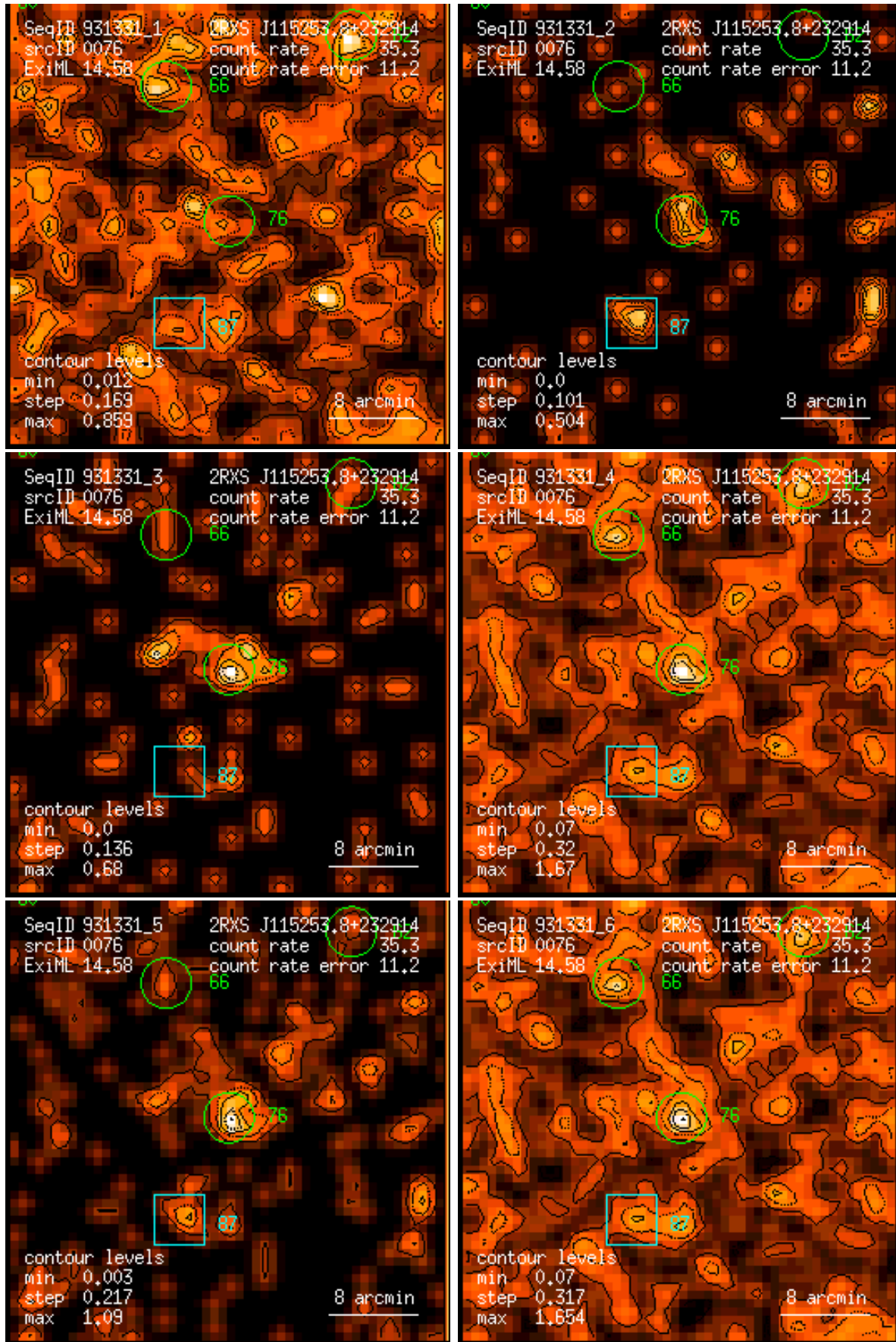
Figure 76: RASS 931331: detection 0076: band rate images, Gaussian filter: (1) PSPC channels 11 – 41, (2) 52 – 90, (3) 91 – 201, (4) 11 – 235, (5) 52 – 201, (6) 11 – 201. Broad band rates in counts/ks. Band rate contour levels in counts/ks/arcmin 2 .
